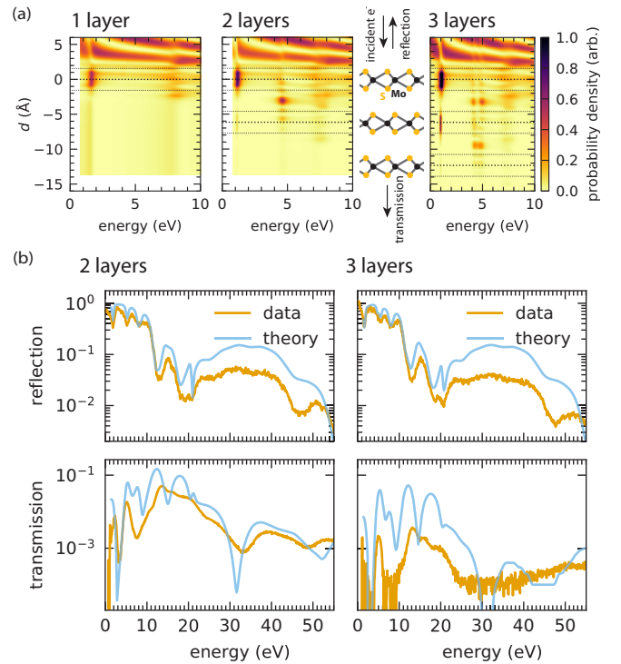
FIG. 2. (a) Calculated probability density along the out-of-plane direction for an electron wave incident from the top for one, two, and three layers of MoS 2 , with the Mo and S planes marked as dotted lines. (b) Comparison of the recorded reflection and transmission (dark count subtracted) spectra and the calculated values. The features of the reflection curves match well. The experimental transmission spectrum appears more broadened as discussed in the text.
