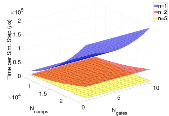
FIGURE 7. Execution time per step for the HH fully featured .
