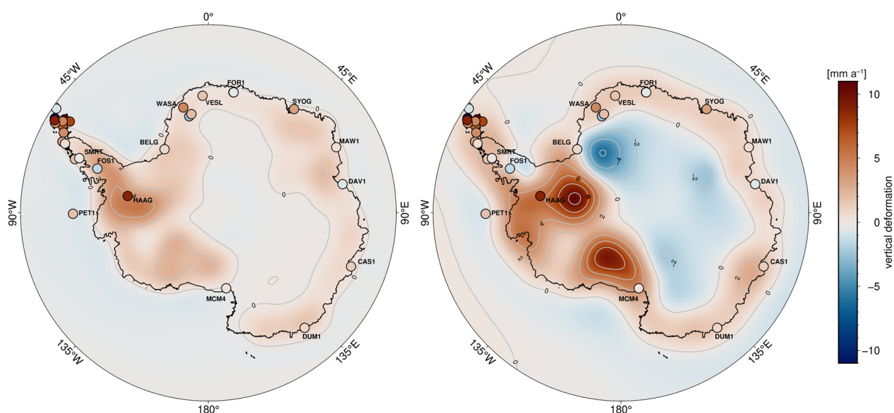
Fig. 6. Vertical deformation rates inferred for selected permanent and campaign GNSS sites in Antarctica (according to Rülke et al. 2015, table 1). The GNSS results were corrected for the present-day elastic uplift. In the background, vertical deformation rates are plotted as predicted by respective GIA models: (left) IJ05_R2 (Ivins et al. 2013); (right) W12a (Whitehouse et al. 2012).
