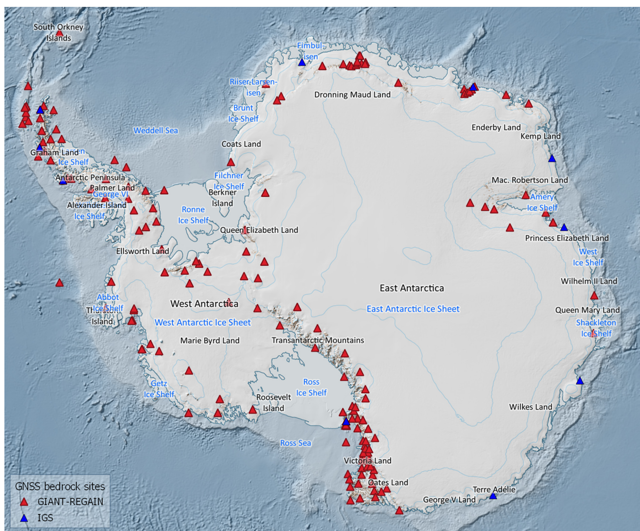
Fig. 5. Distribution of permanent and episodic GNSS sites in Antarctica used in the GIANT-REGAIN reprocessing (red triangles). Blue triangles denote IGS sites.
