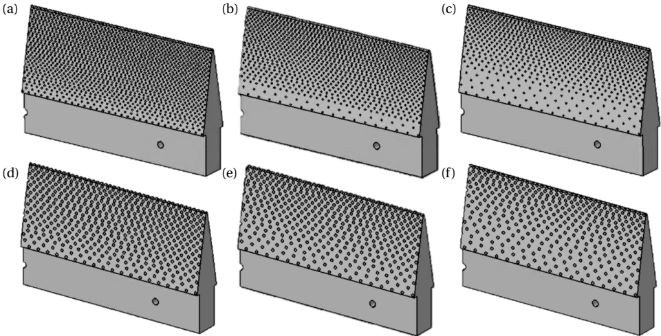
Figure 7.5: CAD drawing of graded trailing-edge mock-ups. Each insert has a span of 10 cm, and a total length of 6 cm. (a) DH08LH20RAD. (b) DH08LH20LIN. (c) DH08LH20EXP. (d) DH14LH25RAD. (e) DH14LH25LIN. (f) DH14LH25EXP.
