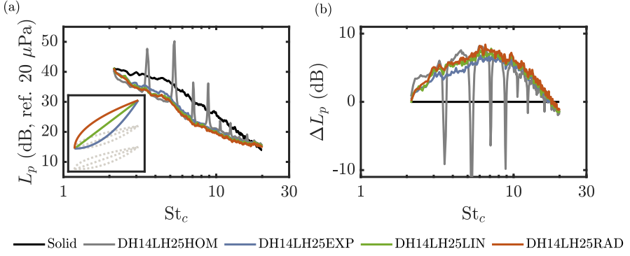
Figure 7.9: Acoustic spectra at a free-stream velocity of 30 m/s with the NACA 0018 model at no incidence. Set of permeable inserts with hole diameter d_h = 1.4 mm and hole spacing at the tip l_{h,tip} = 2.5 mm. (a) Absolute levels. The permeability distribution of the graded inserts is highlighted in the left bottom corner plot. (b) Relative spectra with respect to the solid case.
