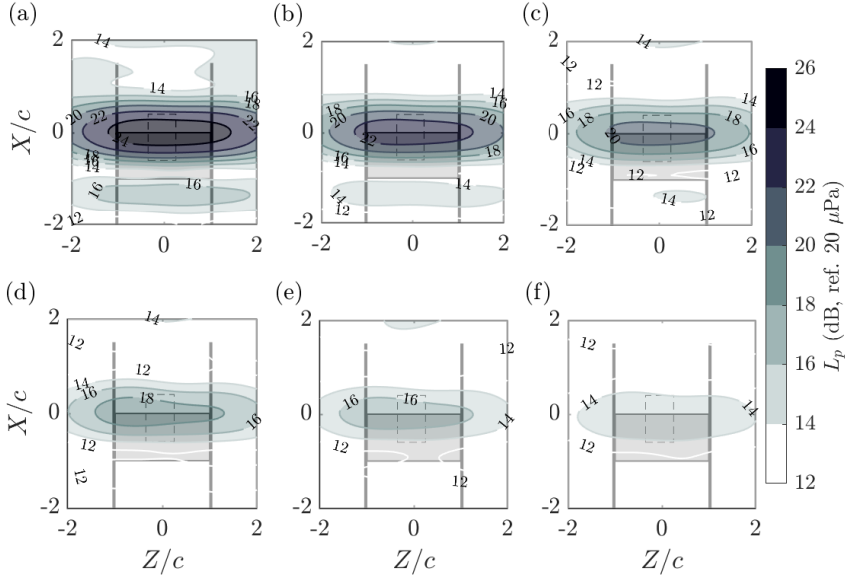
Figure 3.20: Acoustic source maps measured at U_\infty = 25 m/s for solid and channelled trailing edges. Source maps correspond to a frequency of 1400 Hz. Integration area is marked by the dashed line. Dynamic range is 14 dB. Permeable inserts cover 20% of the chord length. (a) Solid. (b) l_h = 5 mm. (c) l_h = 3 mm. (d) l_h = 2.5 mm. (e) l_h = 2 mm. (f) l_h = 1.5 mm.
