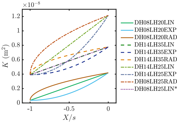
Figure 7.1: Imposed permeability distributions along the chord of the flow permeable trailing-edge inserts. Sample code with "*" refers to NACA 63018, others to NACA 0018.
