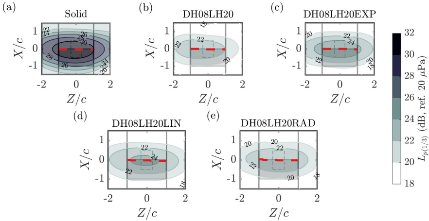
Figure 7.7: Source maps for f = 1000 Hz ( St_c = 7 ) for the NACA 0018 trailing-edge inserts with l_h = 0.8 mm and l_{h,tip} = 2 mm. (a) Solid. (b) DH08LH20HOM. (c) DH08LH20EXP. (d) DH08LH20LIN. (e) DH08LH20RAD. The airfoil is represented as a gray rectangle. Dashed area represents the region where the source power integration technique is applied. Red dashed-dotted line marks streamwise L_p maxima within -1 < Z/c < 1 .
