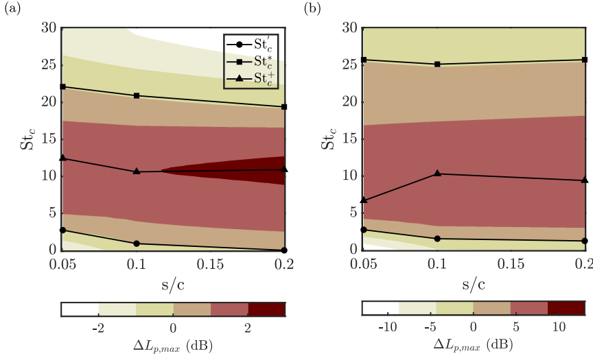
Figure 6.12: Change in maximum noise attenuation \Delta L_{p,\max} with permeable chordwise length s/c and chord-based Strouhal number St_c for perforated inserts with l_h = 5 (a) and 2 mm (b) at \alpha = 0.2 degrees.
