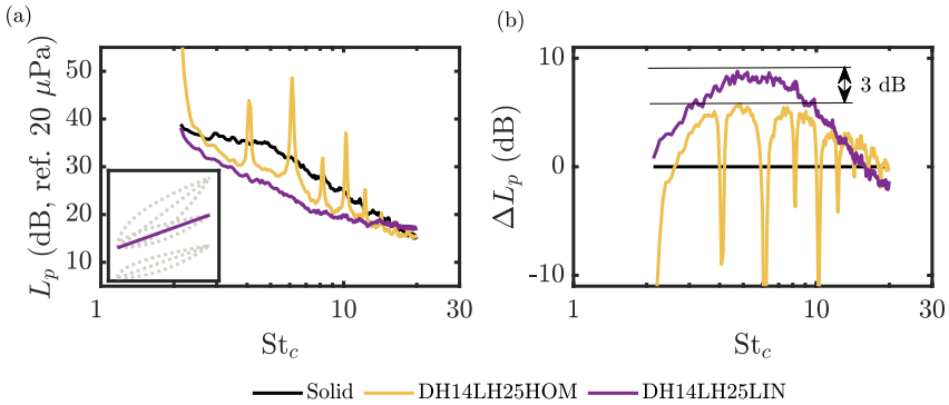
Figure 7.10: Acoustic spectra measured for the set of permeable inserts with hole diameter d_h = 1.4 mm and hole spacing at the tip l_{h,tip} = 2.5 mm. Data measured at a free-stream velocity of 30 m/s with the NACA 63018 model at no incidence. (a) Absolute spectra. The permeability distribution of the graded insert is highlighted in the left bottom corner plot. (b) Relative spectra with respect to the baseline case.
