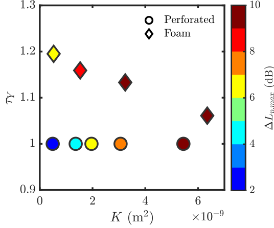
Figure 6.9: Maximum noise attenuation \Delta L_{p,max} as a function of permeability K and tortuosity \tau_Y for \alpha = 0.2 deg.
