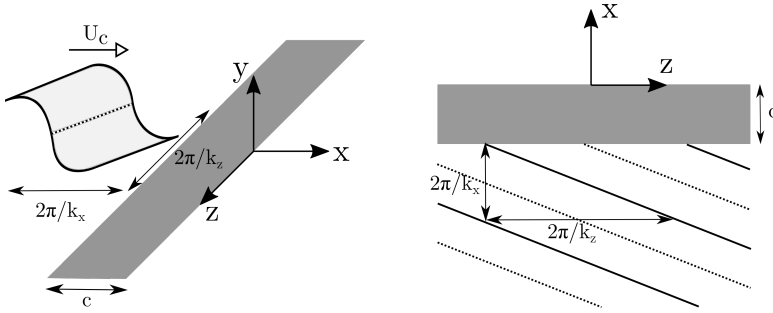
Figure 2.4: Sketch depicting a flat plate with an 3D incident gust.
