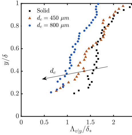
Figure 4.8: Variation of \Lambda_{v|y}/\delta_* across the boundary layer at U_\infty = 20 \text{ m/s} and x/c = -0.02 . Data obtained with PIV configuration A.
