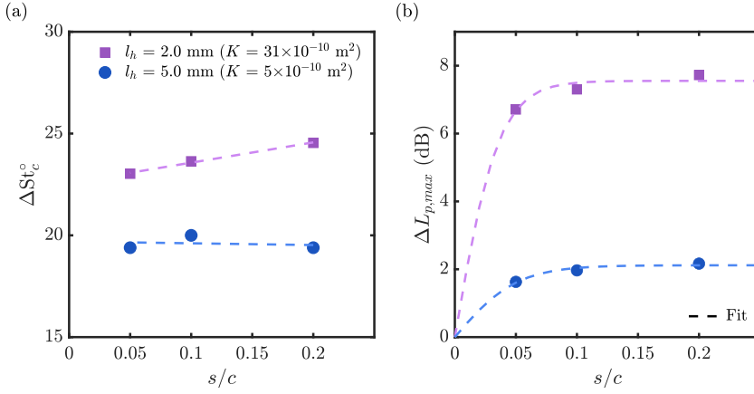
Figure 6.13: Change in the frequency range for noise mitigation \Delta St_c^\circ (a) and maximum noise attenuation \Delta L_{p,max} (b) with permeable chordwise length s/c for perforated inserts with l_h = 2 and 5 mm ( \alpha = 0.2 deg.).
