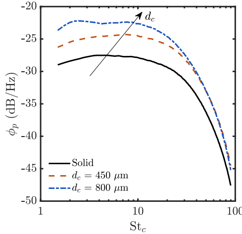
Figure 4.10: Power spectral density of surface pressure \phi_p measured at a U_\infty = 20 \text{ m/s} for solid and metal foam trailing edges.
