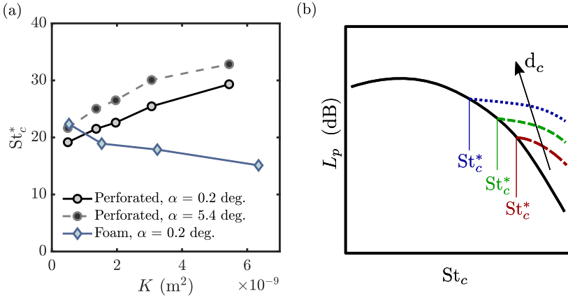
Figure 6.7: (a) Change in St_c^* with permeability for perforated and metal foam inserts at \alpha = 0.2 and 5.4 degrees. (b) Sketch depicting typical roughness noise features for porous edges. Black line represents baseline (smooth surface) trailing-edge noise. Dashed lines illustrate roughness noise contributions for increasing pore size d_c , i.e. higher roughness.
