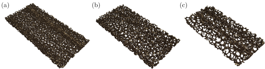
Figure 3.10: CT-scanned samples (resolution: 12 \text{ }\mu\text{m} ) of metal foams with different pore size and permeability. Size: 10 \times 5 \times 0.5 \text{ mm}^3 . (a) d_c = 450 \text{ }\mu\text{m} . (b) d_c = 580 \text{ }\mu\text{m} . (c) d_c = 800 \text{ }\mu\text{m} .
