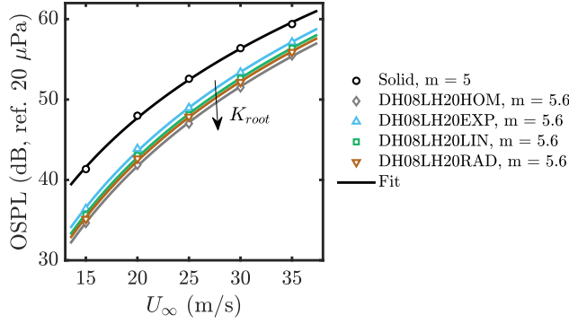
Figure 7.12: Change in OSPL with free-stream velocity for the set of permeable inserts with hole diameter d_h = 0.8 mm and hole spacing at the tip l_{h,tip} = 2 mm. Data measured at a free-stream velocity of 15 to 35 m/s with the NACA 0018 model at no incidence. Markers represent measured data; lines depict fitted data employing the equation 6.3.
