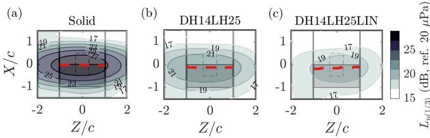
Figure 7.11: Source maps for f = 900 Hz ( St_c = 6 ) for the NACA 63018 trailing-edge inserts with l_h = 1.4 mm and l_{h,tip} = 2 mm. (a) Solid. (b) DH14LH25HOM. (c) DH14LH25LIN. The airfoil is represented as a gray rectangle. Dashed area represents the region where the source power integration technique is applied. Red dashed-dotted line marks streamwise L_p maxima within -1 < Z/c < 1 .
