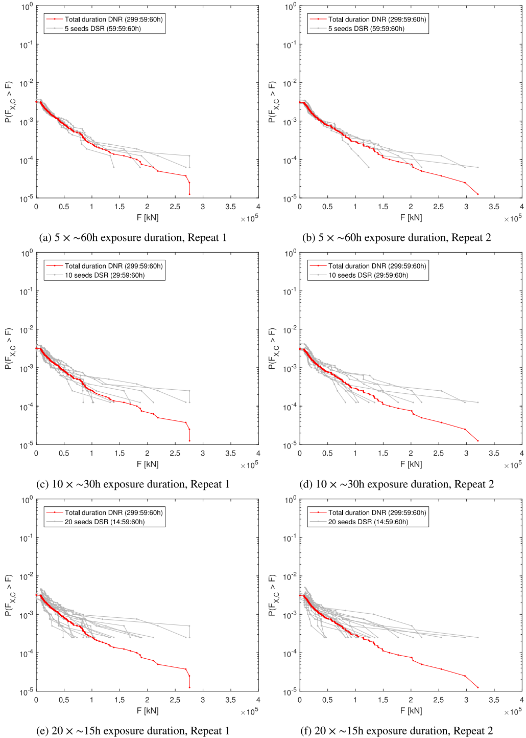
Fig. 6. DSR and DNR distributions of total wave impact force peaks on deck box F_X , for different exposure durations and number of seeds.
