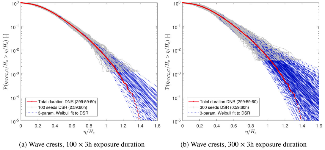
Fig. B.13. DSR and DNR distributions of \eta_{WCLC} for different exposure durations and number of seeds. Including 3-parameter Weibull fits to top 30% crests in the DSR distributions.
