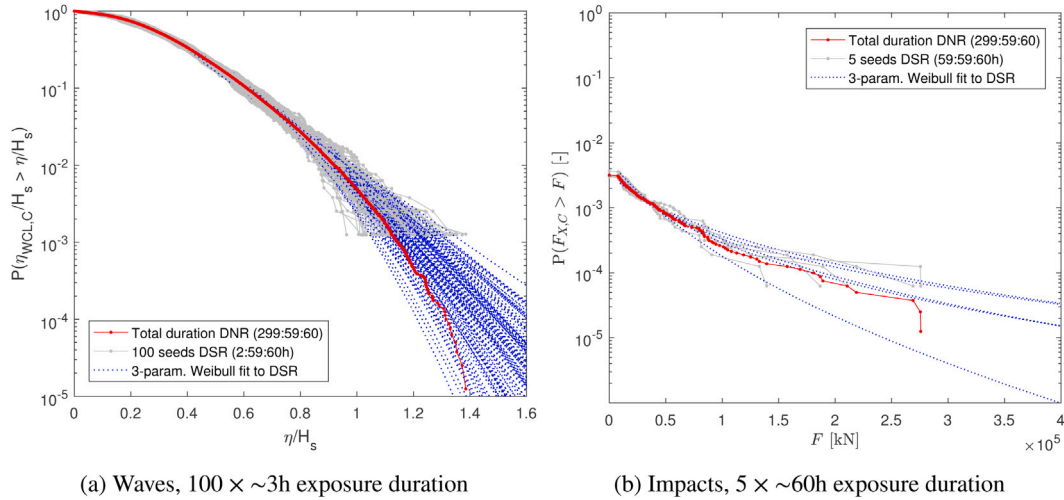
Fig. 8. DSR and DNR of \eta_{WCLC} (left) and F_{XC} (right), crests for 3 h exposure duration, impact loads for 60 h exposure duration. Including 3-parameter Weibull fits to top 30% crests (waves) or top 90% peaks (forces) in the DSR distributions.
