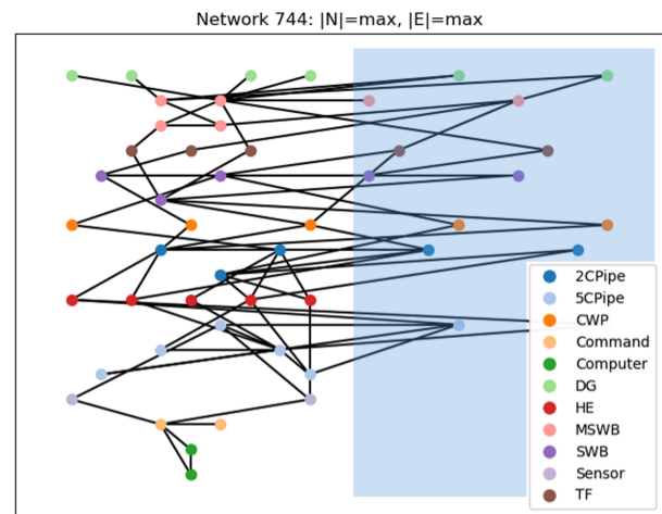
Figure 5: Generated network 744 (also shown in Figure 3) with the maximum number of nodes |V|_{\max} = 50 and edges |E|_{\max} = 77 . With 14 additional nodes (highlighted in the blue box), the maximum of 20 additional nodes is not part of the generated network set.
