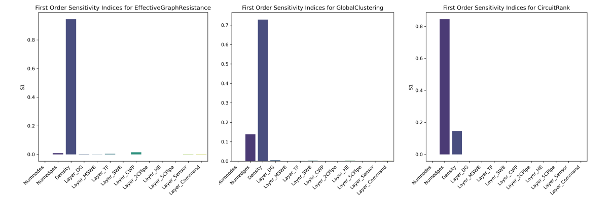
Figure 8: First order sensitivity analysis of the network robustness metrics Effective graph resistance, Global clustering and Circuit rank. The higher-order sensitivity analysis shows marginal values and is therefore not shown in this paper. The sample size of this analysis is set to N = 2E15, D = 13 .
