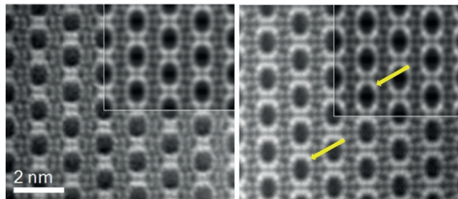
Figure 2. ADF-STEM images along [100] of as-prepared \text{AlPO}_4 STA-28 (left) and \text{FeAlPO}_4 STA-28 (right) processed as described in the SI, section S11, to give an averaged image. QSTEM simulations in which 0% and 75% of “Al(5)”, respectively, have been replaced by Fe are inset. Arrows indicate representative positions of Fe atoms in experimental and simulated images.
