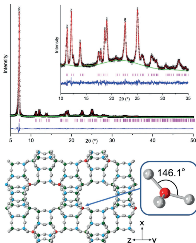
Figure 3. Above: Rietveld refinement plot of calcined, dehydrated \text{FeAlPO} STA-28, R_{\text{wp}} = 0.038 ; below: measured \text{FeAlPO} STA-28 framework and, inset, DFT modelled geometry around the \text{Fe}^{3+} .
