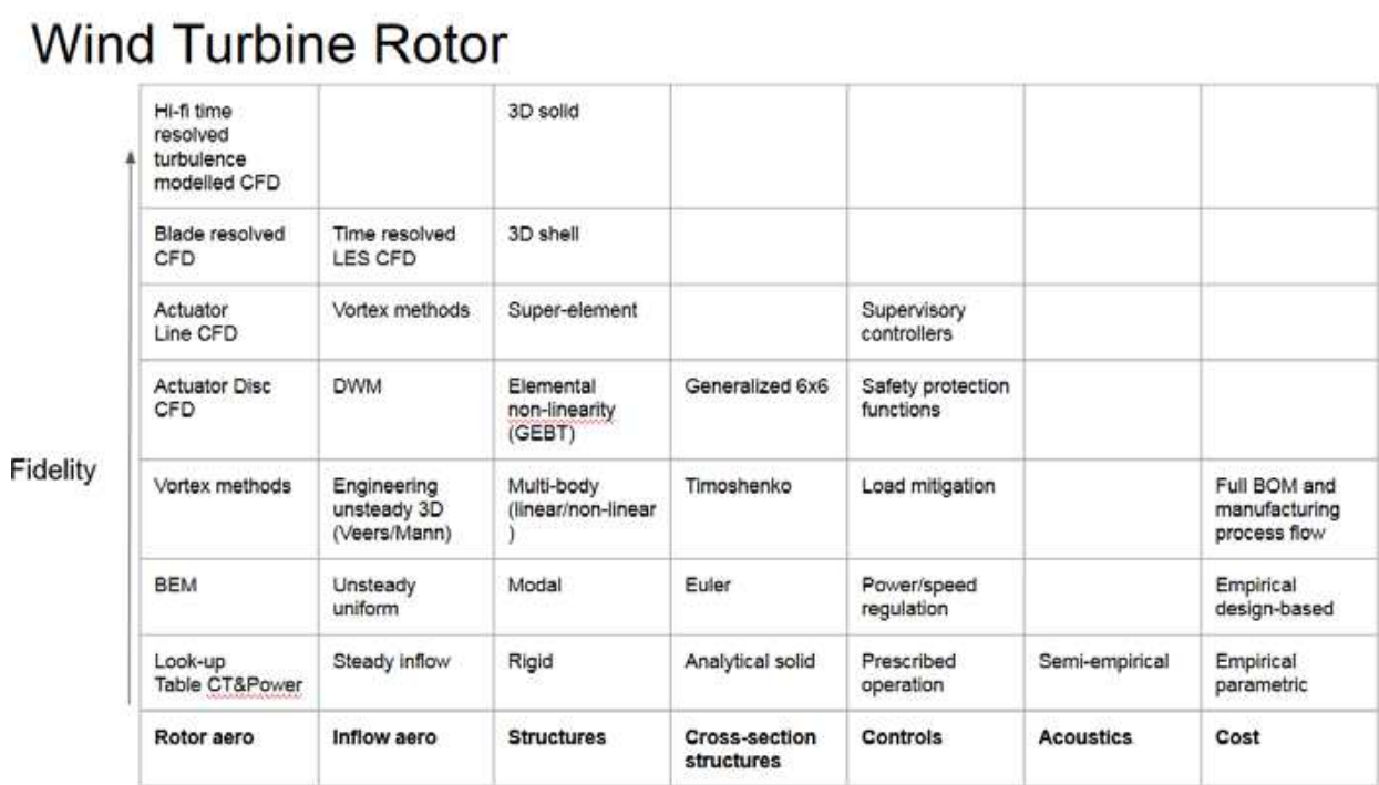
Figure 1: Draft Discipline-Fidelity Matrix for the Wind Turbine Rotor; this has been cross-walked against existing MDAO frameworks for wind turbine rotors. The most common fidelities for each discipline are identified and are the starting point for ontology development (i.e. Blade-Element Momentum (BEM) for rotor aerodynamics).
