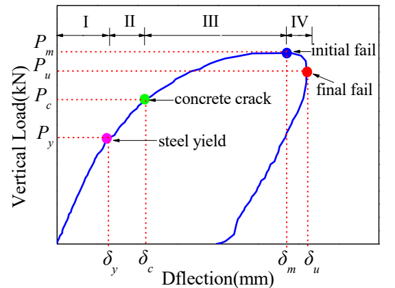
Figure 4. Vertical load-deflection response
