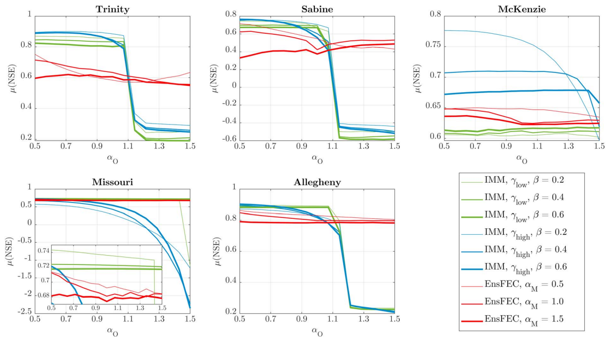
Figure 12. \mu(\text{NSE}) values obtained for different values of the coefficient \alpha_O on the five river reaches in case of low and high values of model error \gamma , various assumption on observation error \beta for IMM method, and three values of coefficient \alpha_M for the FEC approach. IMM = Interacting Multiple Model; FEC = Fuzzy Error Correction; NSE = Nash-Sutcliffe efficiency.
