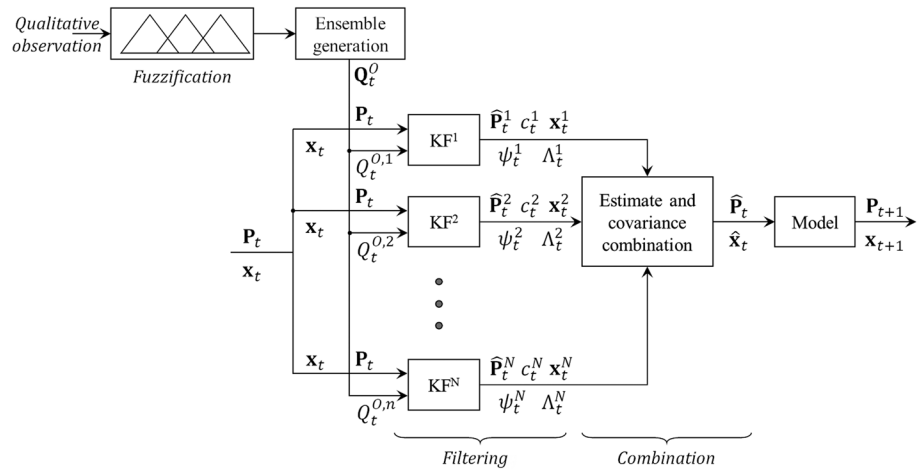
Figure 3. Schematic representation of the modified IMM procedure with both filtering and combination steps reported. In particular, P indicates the error covariance matrix, x is the model state, Q^O the ensemble of fuzzy observations, c is a normalizing factor, \Lambda the likelihood of the observations, \psi is the probability of each filter KF, where the superscript number indicates the ensemble member. IMM = Interacting Multiple Model; KF = Kalman filter.
