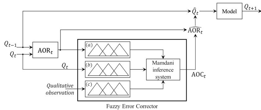
Figure 4. Schematic representation of the output updating method, where Q is the simulated flow, AOR is the angle of rotation, AOC is the angle of correction, and \bar{AOR} is the updated angle of rotation.
