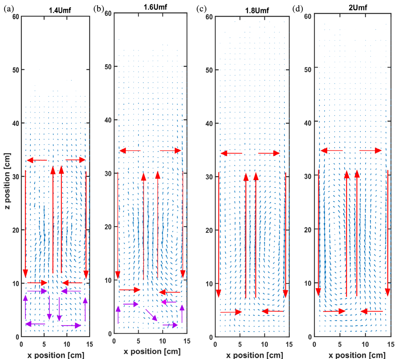
FIGURE 4 Velocity distributions for AR-1 particles in the x-z plane for different gas inlet velocities. Positions are indicated in cm. Red and purple arrows indicate the directions of the main vortices [Color figure can be viewed at wileyonlinelibrary.com ]
