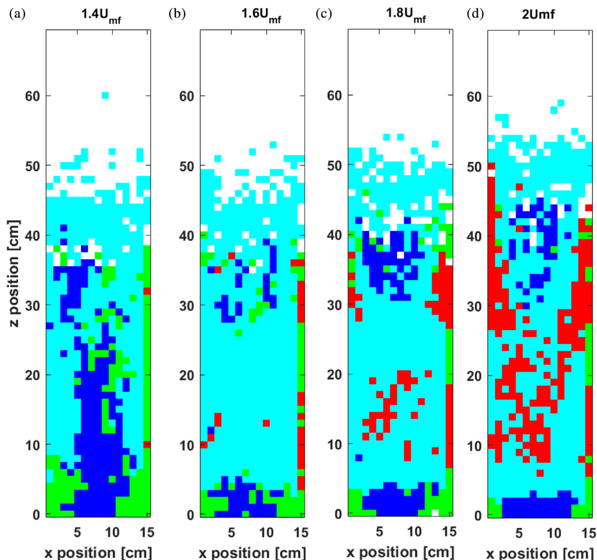
FIGURE 12 Distribution of the predominant orientation of AR-4 particles in the x-z plane. Here the colour scheme is: blue squares (■) are x-aligned, green squares (■) are y-aligned, red squares (■) are z-aligned, and cyan squares (■) are randomly oriented. White space represents empty cells. Schematic representation of color scheme is shown in Figure 13 [Color figure can be viewed at wileyonlinelibrary.com ]
