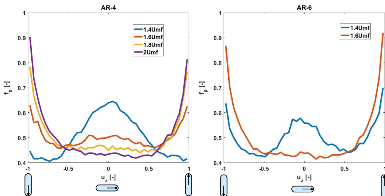
FIGURE 10 Effect of gas velocity on the time-averaged fraction ( f_p ) of particle orientation in the z-direction ( u_z ) of AR-4 and AR-6 particles [Color figure can be viewed at wileyonlinelibrary.com ]
