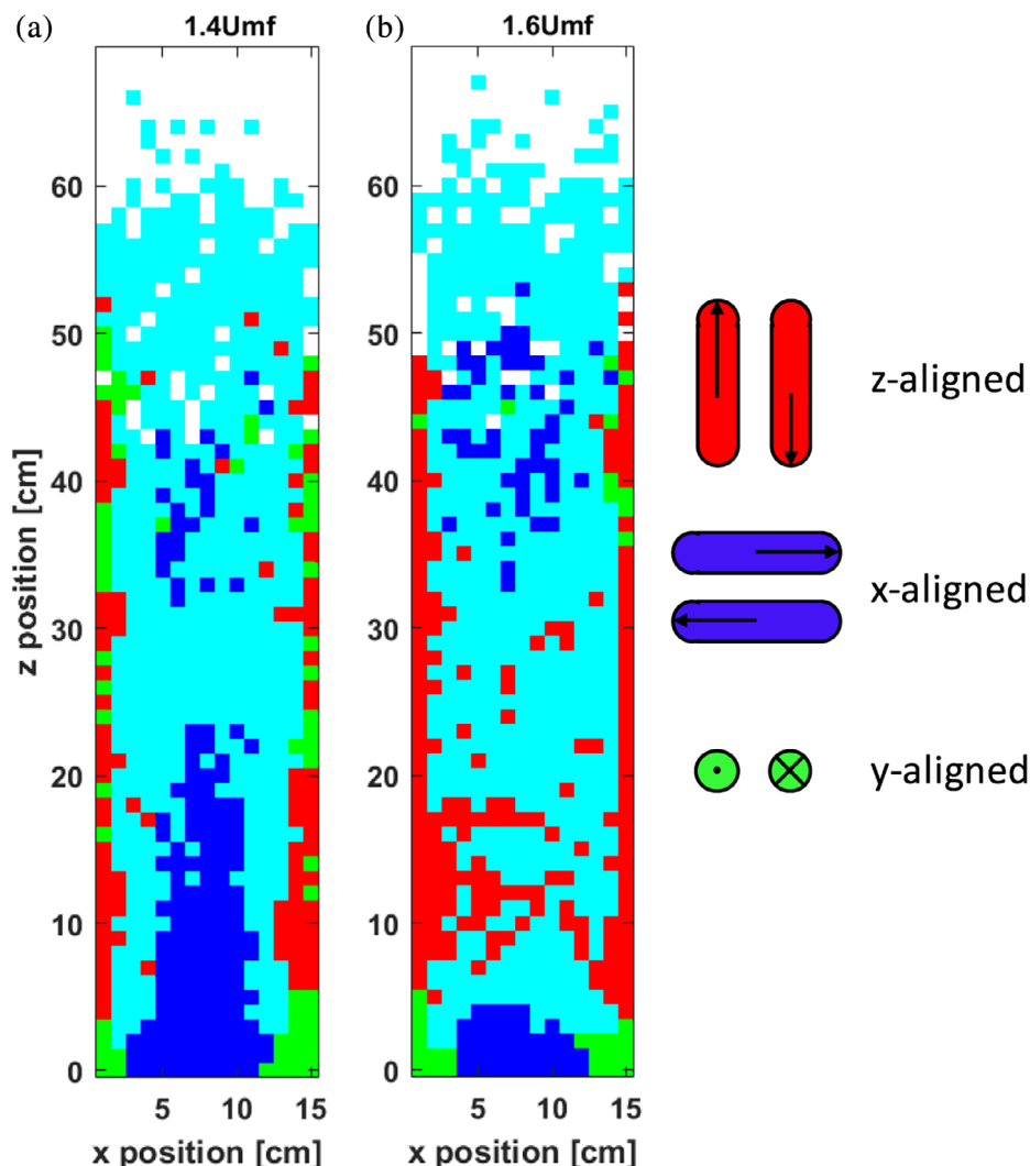
FIGURE 13 AR-6 particle preferred orientation in x-z plane. Here the colour scheme is: blue squares (■) are x-aligned, green squares (■) are y-aligned, red squares (■) are z-aligned, and cyan squares (■) are randomly orientated. White space represents empty cells [Color figure can be viewed at wileyonlinelibrary.com ]
