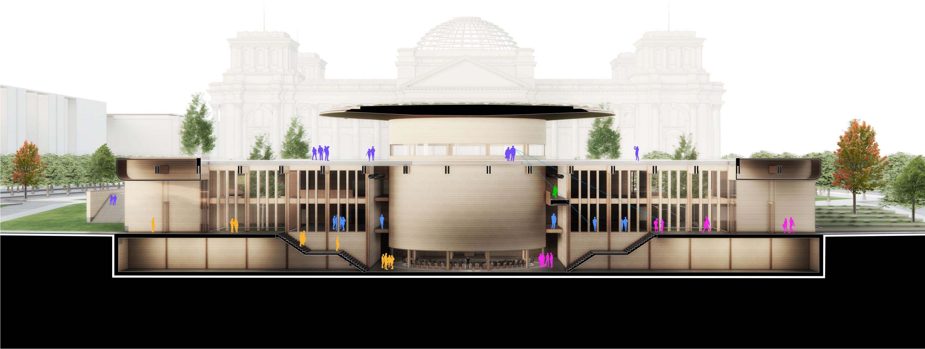
Cross section - Entrance hall
