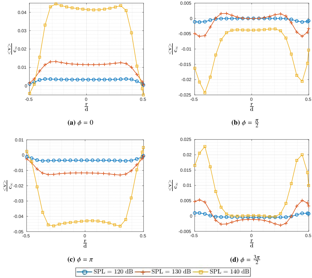
Fig. 16 Phase averaged velocity ( \langle v \rangle ) at the mid-plane of the orifice with change in SPL of the grazing waves at f = 2 \text{ kHz} .
