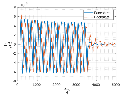
(c) SPL = 150 dB
