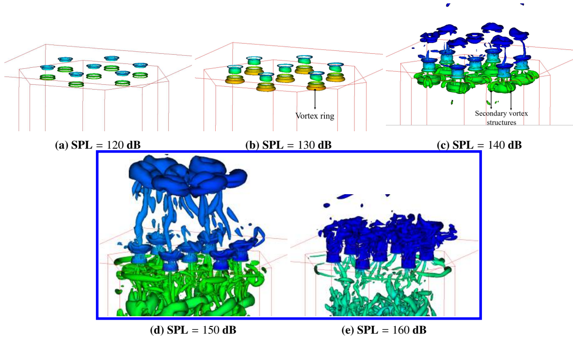
Fig. 15 \lambda_2 iso-surfaces of the induced flow-fields at different SPLs of the grazing waves with f = 2 kHz.
