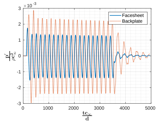
(b) SPL = 140 dB
