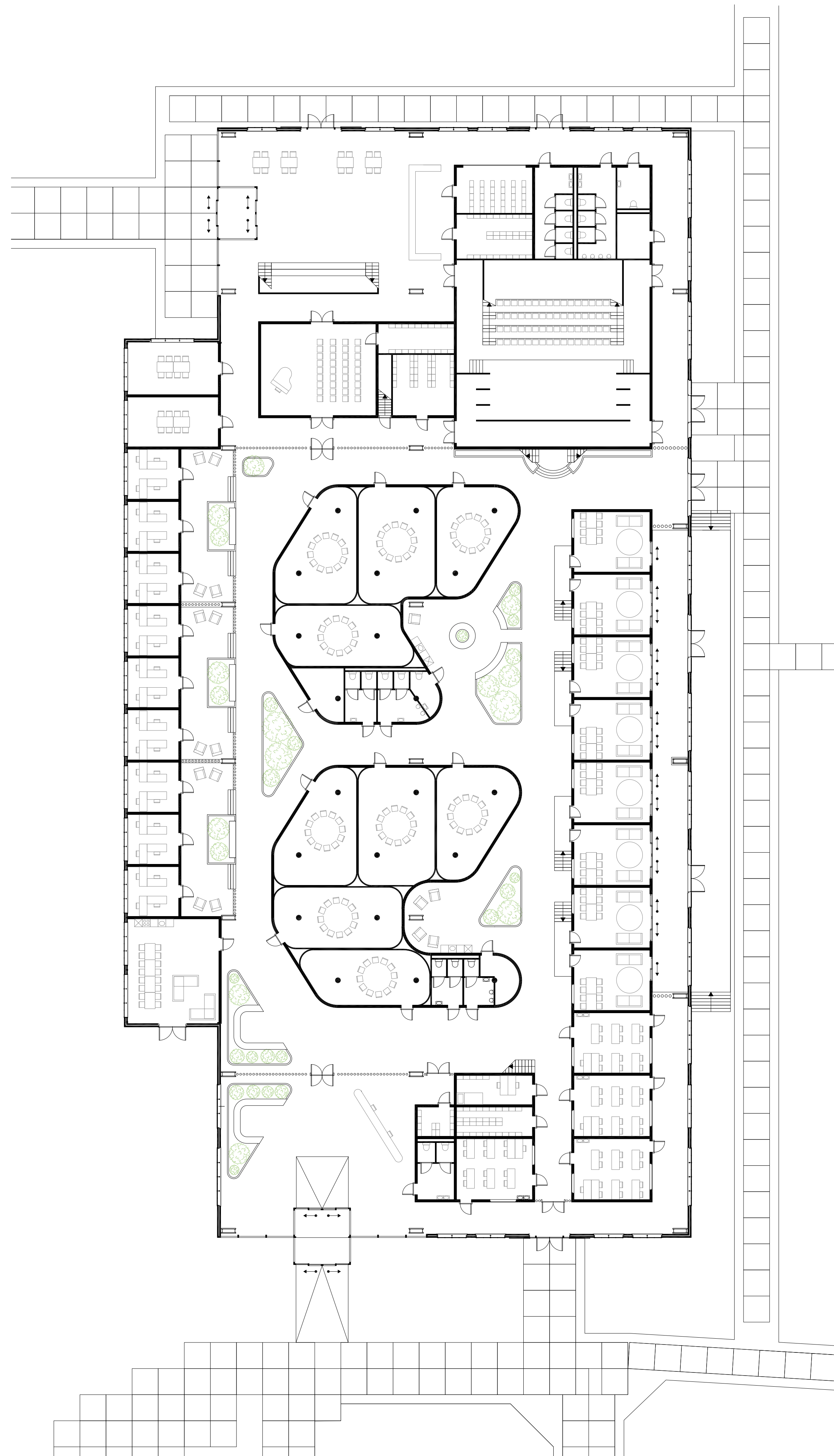
Ground Floor 1:200
