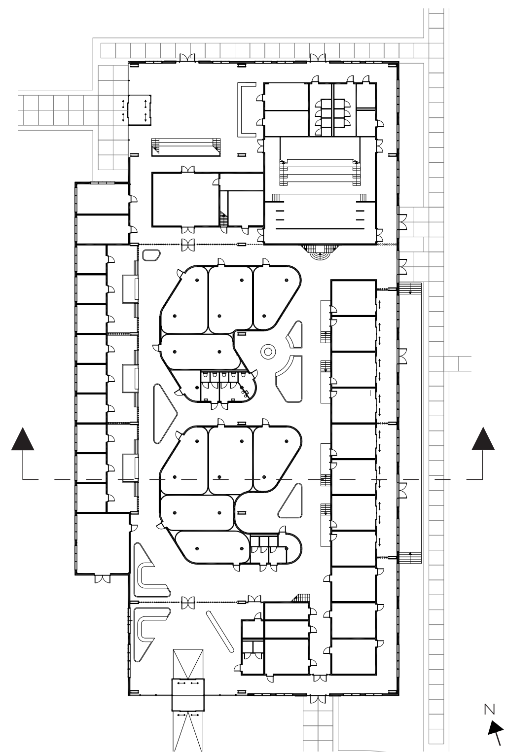
Ground floor 1:500
