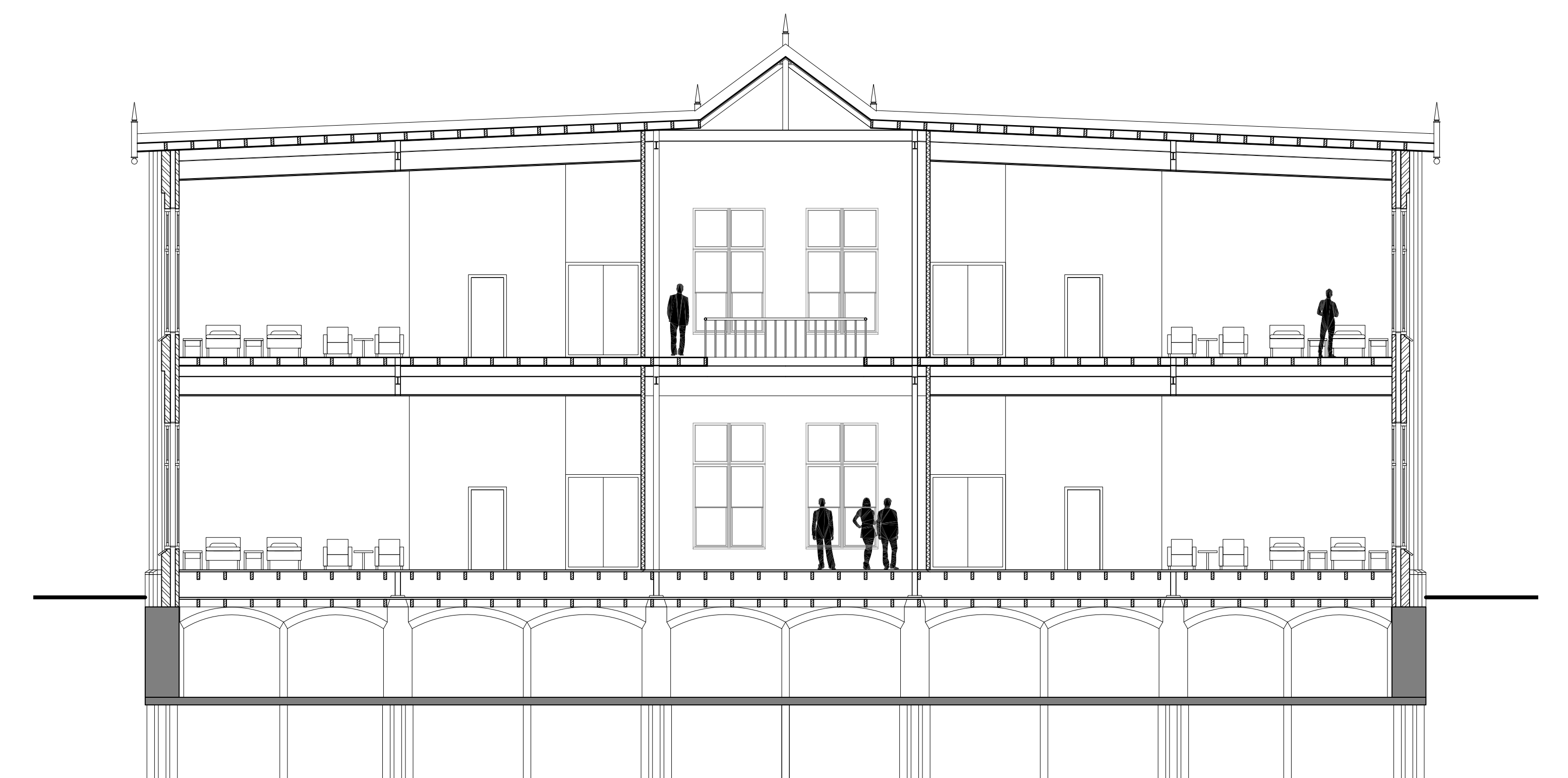
Section 1:100
