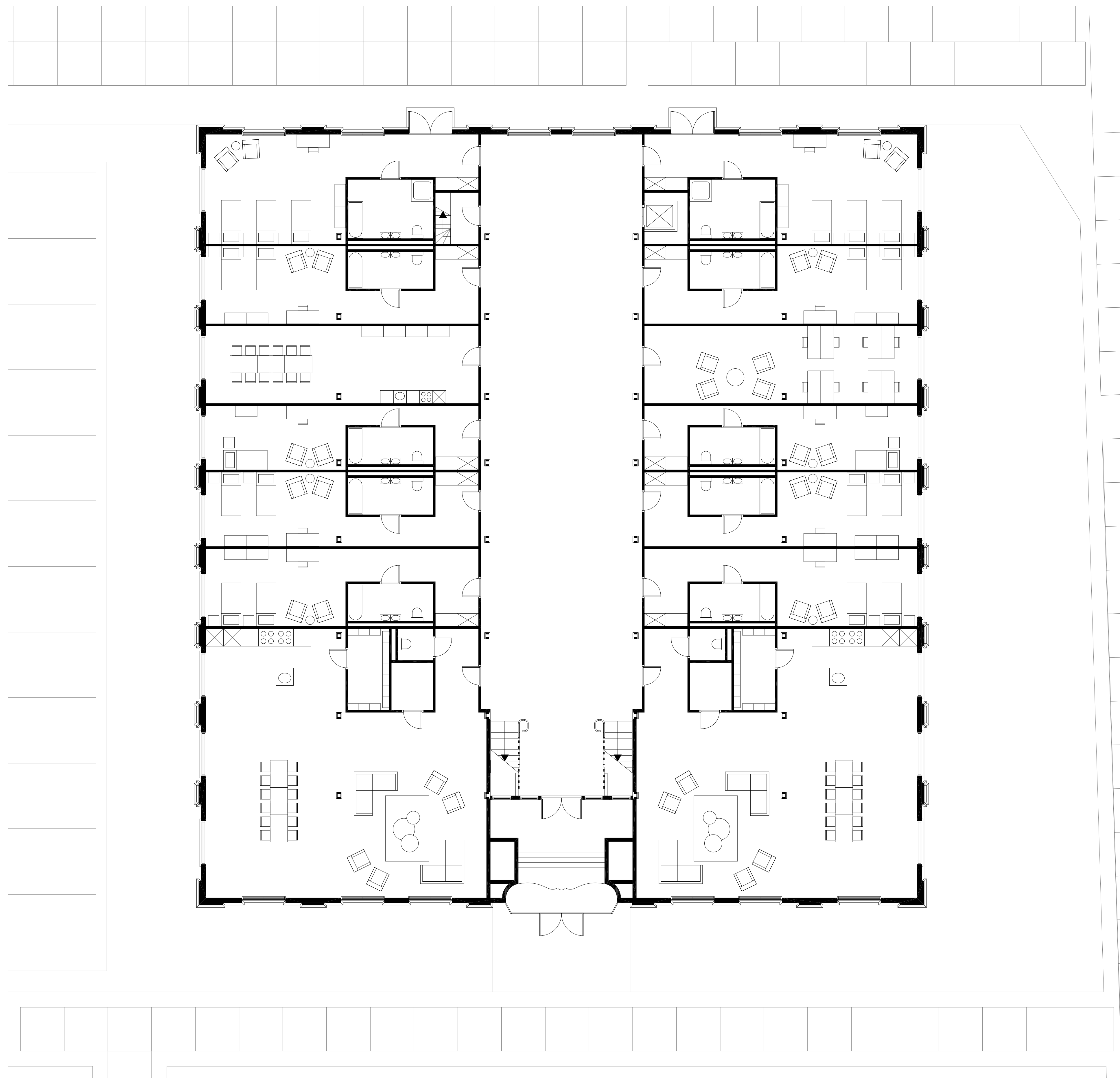
Ground Floor 1:100
