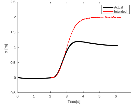
Figure 8: Simulation flight test 1 Trajectory 1, x-position intended-actual comparison
