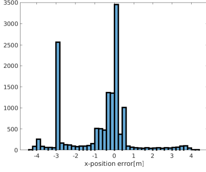
Figure 16: Real world flight test 2, x-position error histogram
