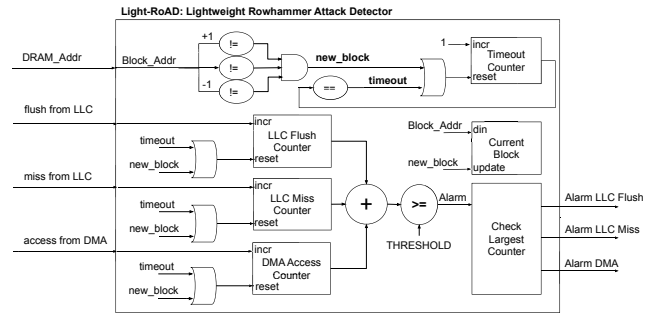
Fig. 1. LightRoAD Architecture
