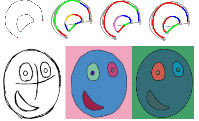
Figure 5: Impact of increasing tolerance \epsilon on fitting cubic Bezier segments ( \epsilon/segment - length = 0.033, 0.05, 0.1px (top left-right); vector output with low and high \epsilon (bottom)).
