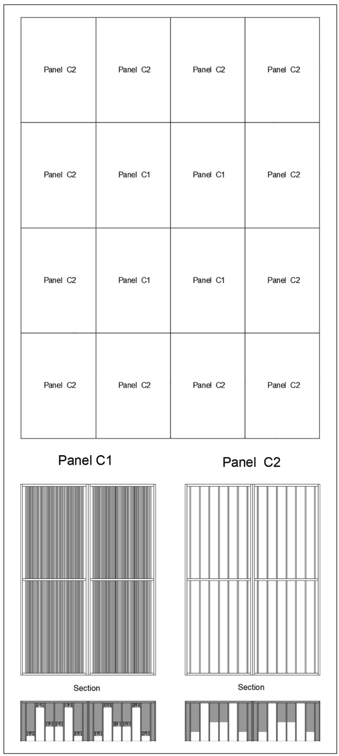
Figure 13. Diffusing panels on the stage.
