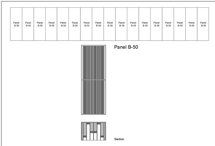
Figure 14. Diffusing panels in the orchestra pit.
