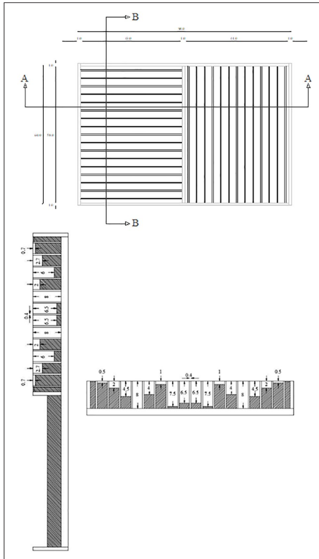
Figure 17. Diffusing panels in the boxes (Section A-A on the left and section B-B on the right).
