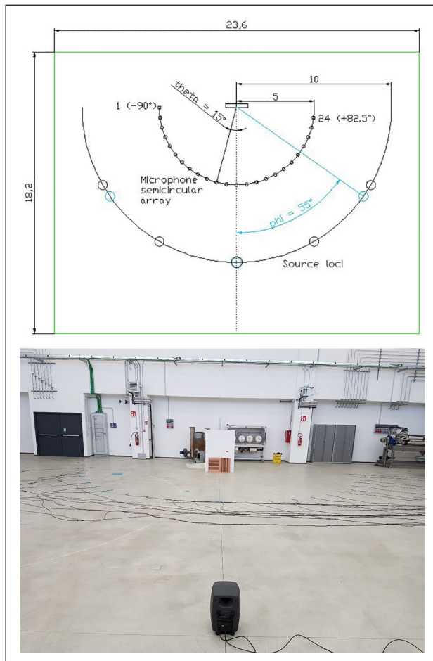
Figure 19. The setting of measurements in the lab on diffusing panels.
