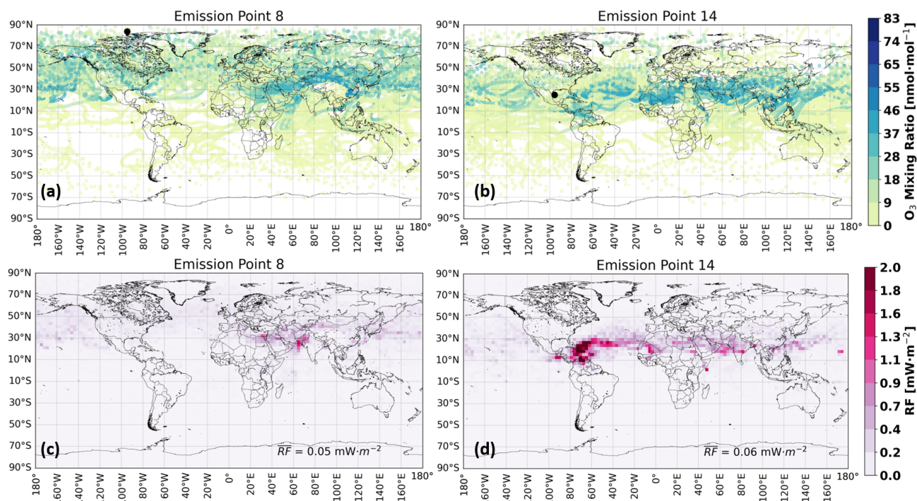
Figure 10. Horizontal profiles of mean O 3 disturbances in N. America in nanomoles per mole ( \text{nmol mol}^{-1} ) during January 2014 for (a) emission point 8 and (b) emission point 14. The mean radiative forcing \overline{RF} in milliwatts per square meter ( \text{mW m}^{-2} ) for (c) emission point 8 and (d) emission point 14. The black dots in (a) and (b) represent the emission starting points.
