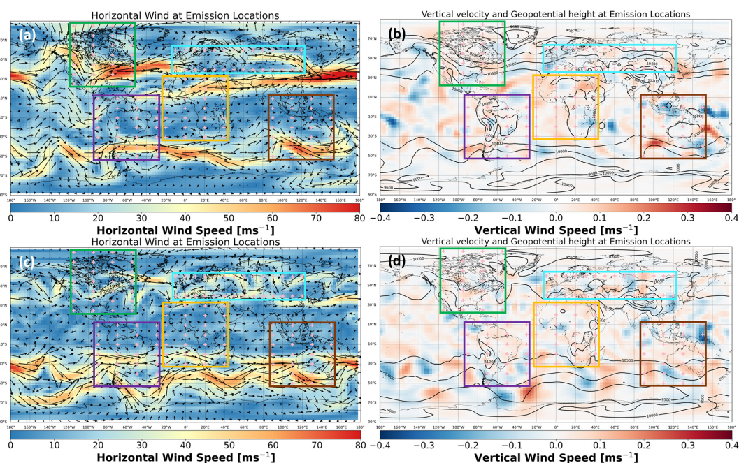
Figure C1. Averaged horizontal and vertical wind fields at \sim 250 hPa during January–March 2014 in panels (a) and (b). Same information is portrayed in panels (c) and (d) for July–September. Geopotential height contours in Fig. C1b and C1d are expressed in meters. The same emission points as in Fig. 1 are shown with “+” in each region.
