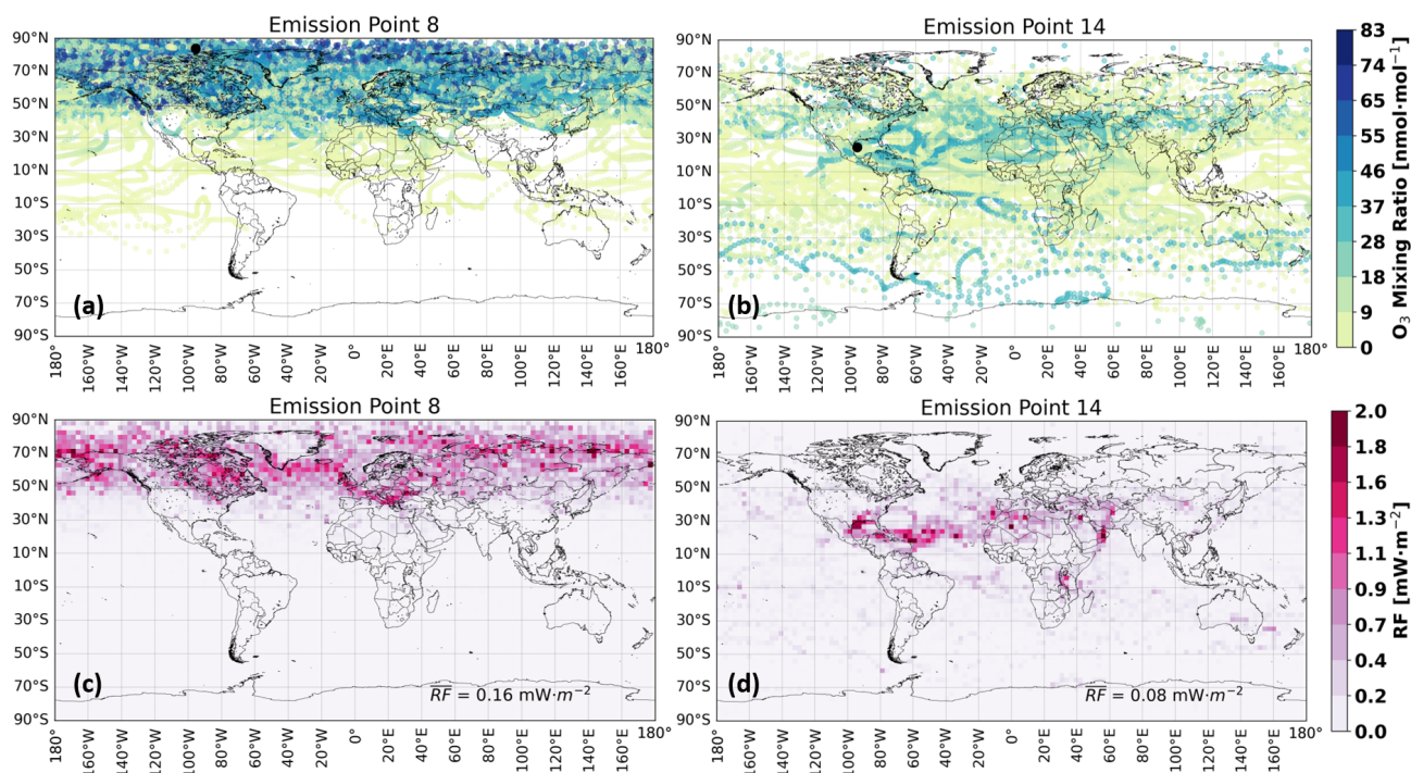
Figure 11. Horizontal profiles of mean O 3 disturbances in N. America in nanomoles per mole ( \text{nmol mol}^{-1} ) during July 2014 for (a) emission point 8 and (b) emission point 14. The mean radiative forcing \overline{RF} in milliwatts per square meter ( \text{mW m}^{-2} ) for (c) emission point 8 and (d) emission point 14. The black dots in (a) and (b) represent the emission starting points.
