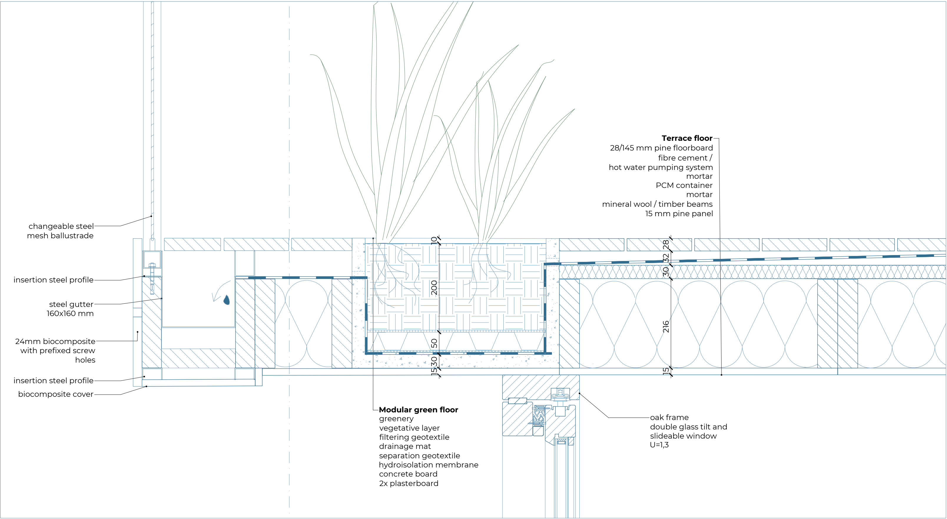
Detail A | Extension module terrace to fence connection
