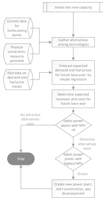
(b) Investment Algorithm
