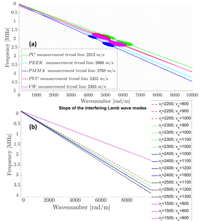
Figure 5. (a) The experimental results obtained with a threshold of -2dB and different materials. (b) The numerical results showing the independency of the Lamb wave method on the shear wave speed of the insonified material.
