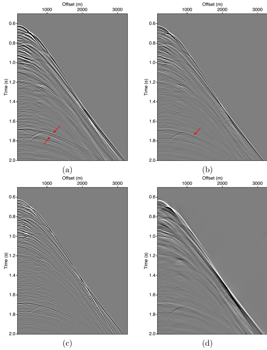
Figure 13: a) Shot record including the source ghost effect as well as the slanted-cable receiver ghost effect. b) Redatumed shot record including the source ghost effect. c) Redatumed shot record including source ghost effect as well as modeled receiver ghost effect. d) Shot record after CNN source deghosting and conventional receiver deghosting.
