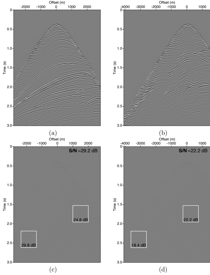
Figure 9: The results of the CNN for one input training shot record and one validation shot record. a) Training shot record (lateral source location: 2925 m) after CNN receiver deghosting. b) Validation shot record with source (lateral source location: 4325 m) after CNN receiver deghosting. c) Difference between Figure ?? and corresponding output training shot record. d) Difference between Figure ?? and corresponding output validation shot record.
