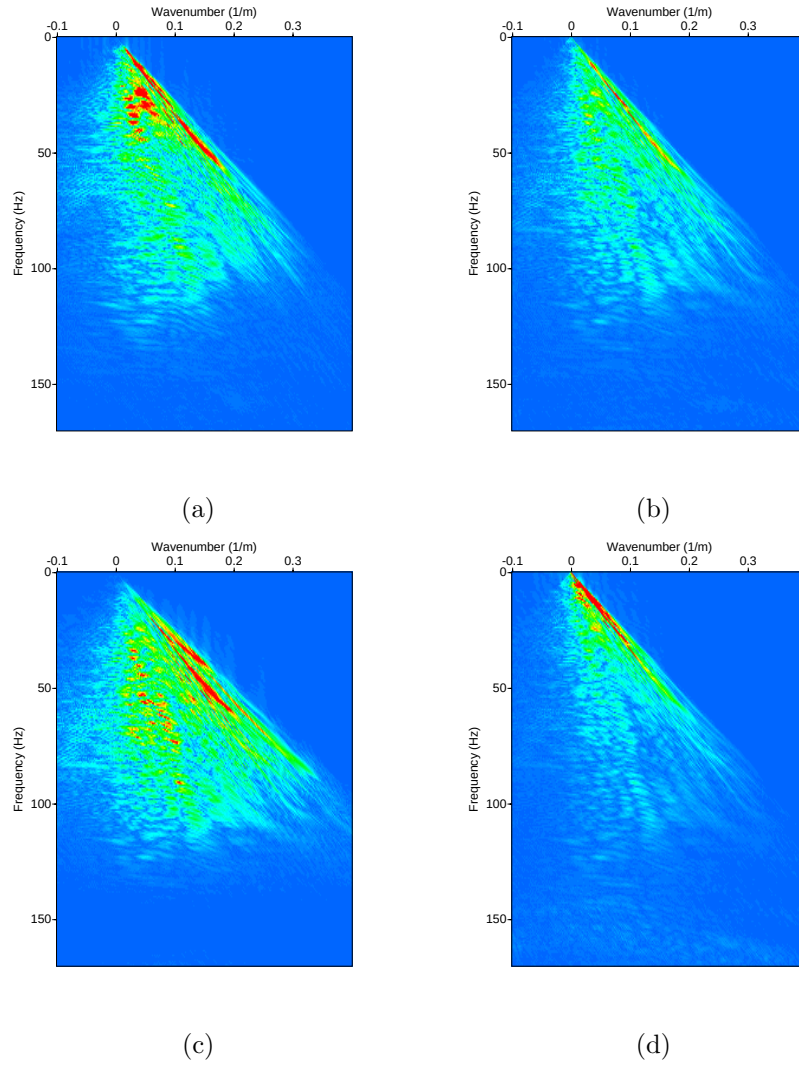
Figure 14: a) The wavenumber-frequency spectrum of Figure 13a. b) The wavenumber-frequency spectrum of Figure 13b. c) The wavenumber-frequency spectrum of Figure 13c. d) The wavenumber-frequency spectrum of Figure 13d.
