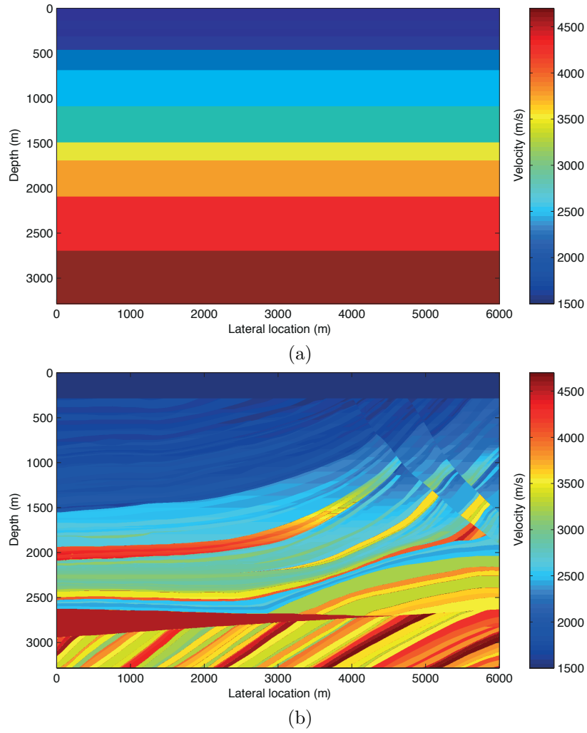
Figure 1: Velocity models used for acoustic finite-difference modeling. a) Velocity model of a laterally invariant subsurface. b) Velocity model of a complex subsurface (Marmousi model including water layer on top).
