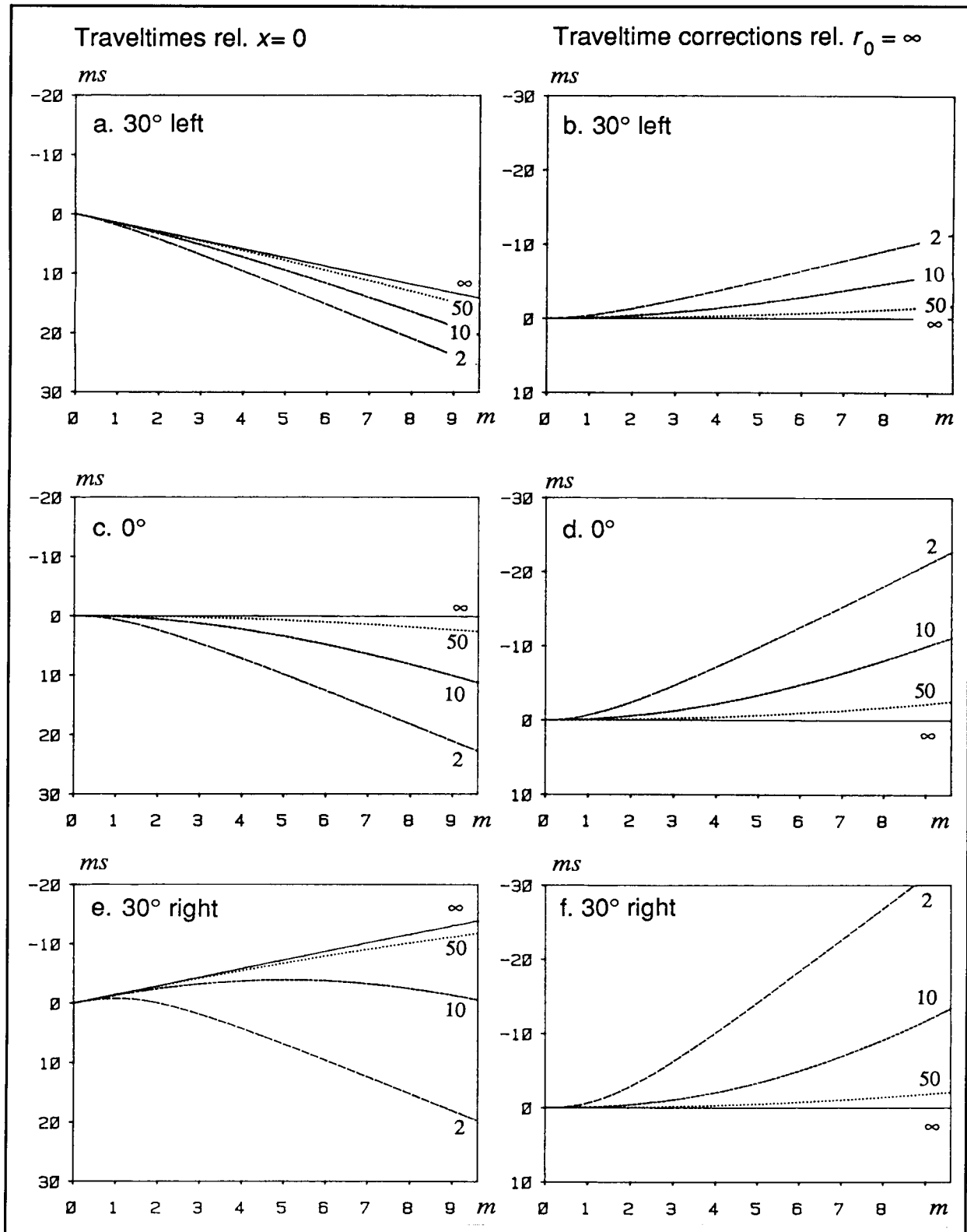
Figure 2.15: Traveltimes along the antenna axis for different source distances and directions. The left figures show the traveltimes differences for source distances of r_0 = \infty , 50, 10 and 2 m and source angles of 30° left, 0° and 30° right. The traveltimes are shown with the axis pointing downwards as is usual in seismics and echoacoustics. The right figures show the necessary traveltime compensation to simulate the Fraunhofer condition.
