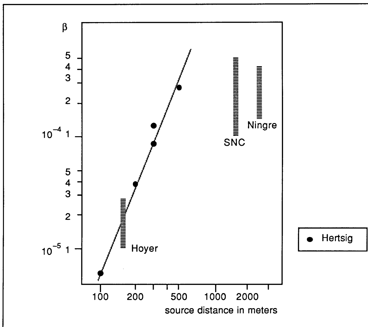
Figure 3.7: The parameter \beta of the coherence function of Eq. (3.24) as a function of the source distance, as measured by Hertsig. Also shown are the range of values found by some investigations, performed at fixed source distances.
