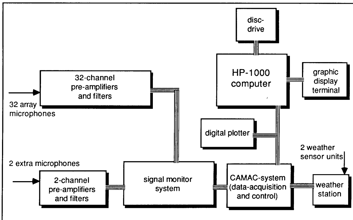
Figure 4.8: Functional block diagram of the data analysis equipment.
