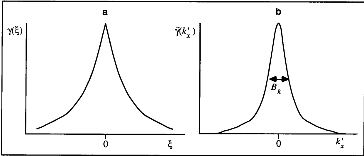
Figure 3.9: a. The transverse coherence function \gamma , according to the model of Ningre [14]; b. its spatial Fourier transform \gamma .
