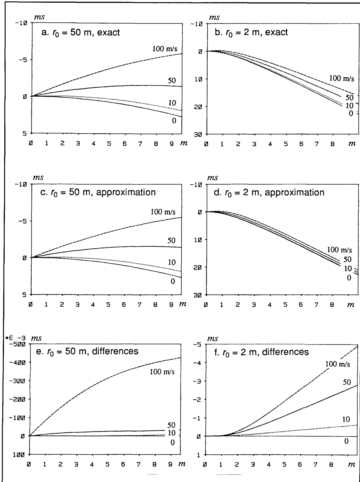
Figure 3.4: Comparison of the exact traveltimes along the antenna axis and the approximation by using c_0 instead of c_{ray} .
