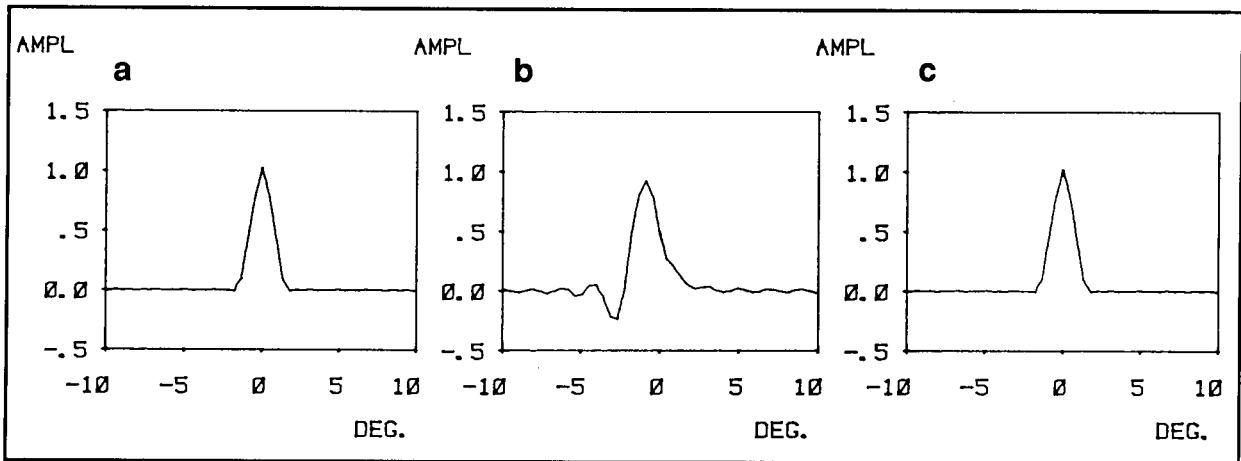
Figure 5.5: The effect of focussing on the beam forming of SYNTACAN for a 1029 Hz source at 0°: a. source at \infty and focus at \infty ; b. source at 200 m and focus at \infty ; c. source at 200 m and focus at 200 m.
