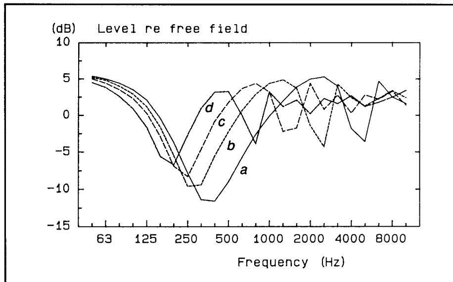
Figure 3.1: The ground effect \Delta L_b for a monopole source at a distance of 200 m and a height of 5 m for different receiver heights: a = 1.5 m; b = 3.0 m; c = 5.0 m and d = 10.0 m (calculations by Koers [28]).
