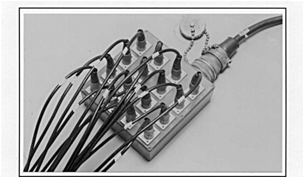
Figure 4.4: One of the connector panels used for the connection of the microphone cables to the multi-channel cables.
