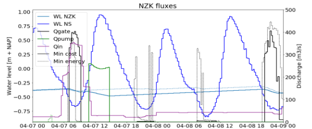
Fig 5 Fluxes of the NZK, scenarios where cost and energy use are minimized
