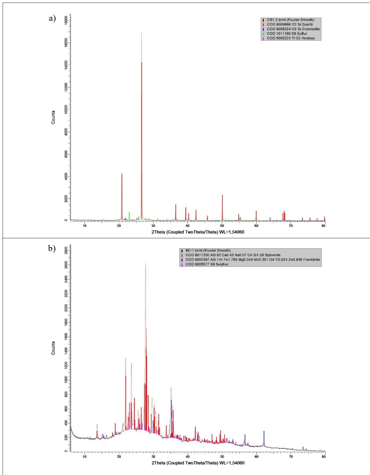
Figure 3. XRD patterns with the peak match and identification. a) sample CB1 where the intense high red peaks have been assigned to quartz. b) BC 1 where the most intense peaks belong to plagioclase. The bumps indicate the amorphous fraction.
