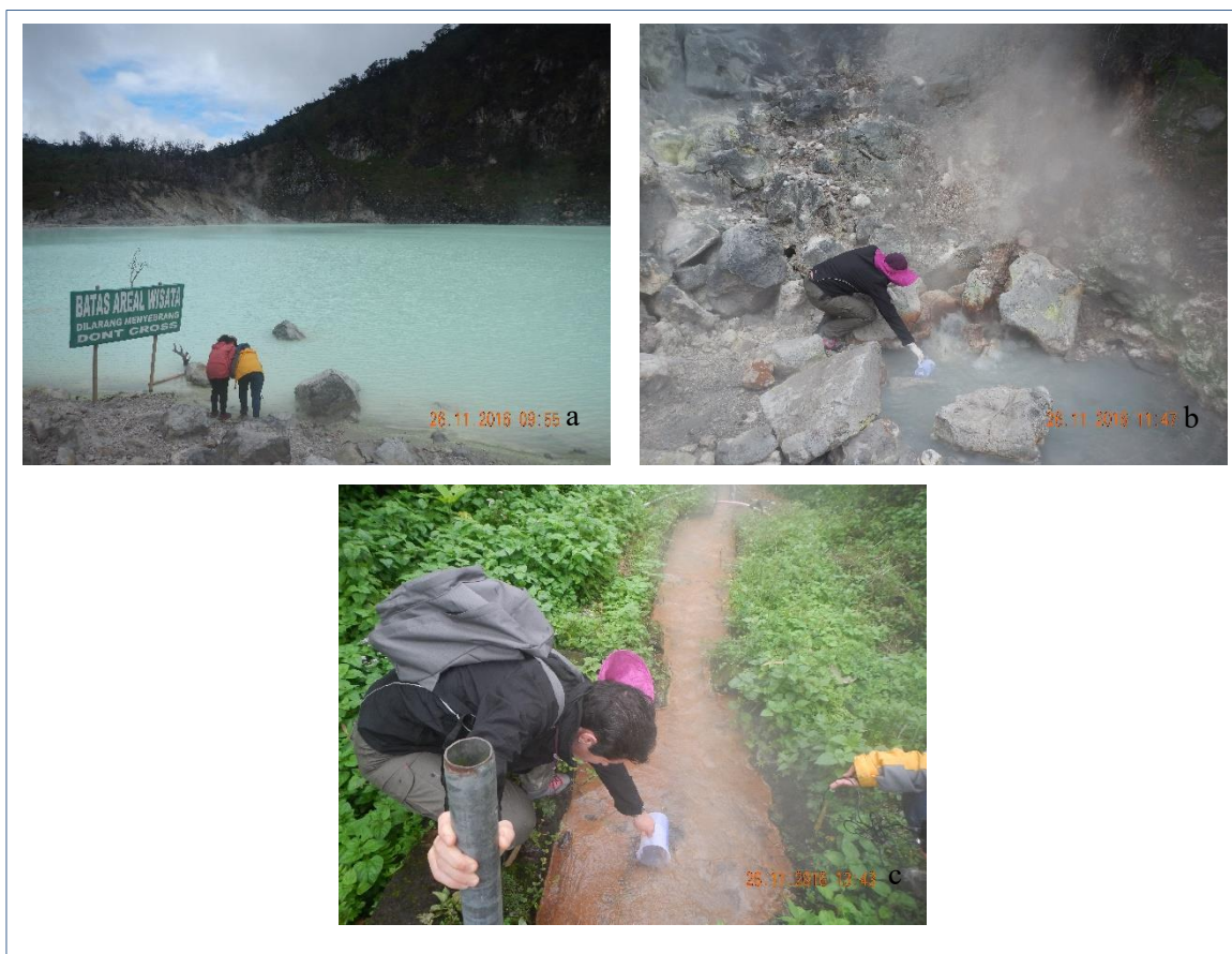
Figure 2. a) acidic volcanic lake crater Kawah Putih. b) hot spring Cimanggu. c) river in Cibolang.
