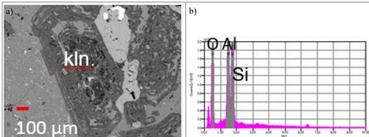
Figure 4. a) EMP image acquired on a plagioclase crystal where the alteration patterns are clearly visible in the plagioclase grain. b) EDS spectrum acquired on the alteration rims showing kaolinite occurrence.
