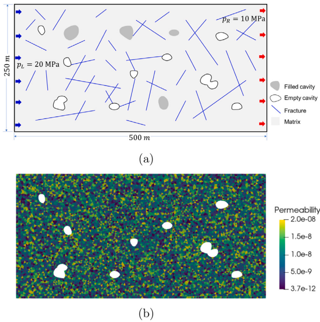
Fig. 19. The large-scale fractured porous medium. (a) Geometry of the model. (b) Permeability distribution (unit: \text{m}^2 ).
