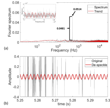
Fig. 4. (a) Fourier spectrum and the trend. (b) Original signal and the despeckling result between 5.25 s and 5.3 s.
