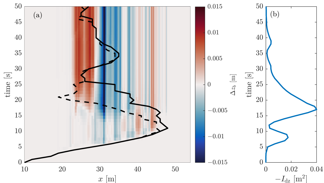
Figure 11. Figure showing the morphological change and runoff (a) and integrated bed level change (b) over time, as predicted by the model. The black lines show the runoff, defined as the maximum position where a certain increase in surface elevation compared with the initial condition is recorded (elevation of 1 cm for the straight line and 2 cm for the dashed line).
