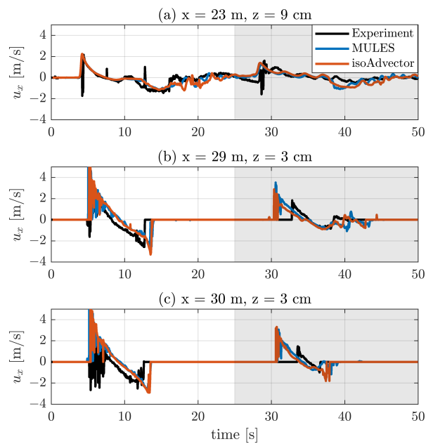
Figure 7. Comparison of cross-shore water velocity u_x between the experiments and two models, using MULES and isoAdvector respectively, at three different cross-locations. Both models use the Engelund and Fredsoe [37] reference concentration model. The last 25 s are shown with a grey background.
