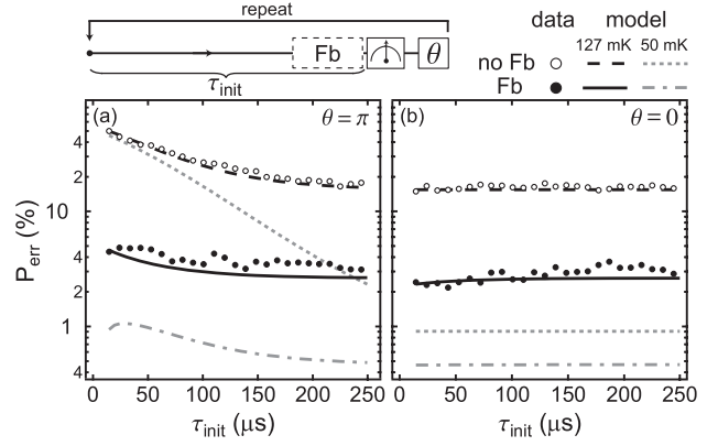
FIG. 4. Fast qubit reset. Initialization errors as a function of initialization time \tau_{init} under looped execution of a simple experiment leaving the qubit ideally in |1\rangle [(a), measurement and \pi pulse] or |0\rangle [(b), measurement only]. Empty circles: Initialization by waiting (no feedback). Solid dots: Initialization by feedback, with three rounds of Fb_0 and a \pi pulse on the 1 \leftrightarrow 2 transition [26]. Curves correspond to a master equation simulation assuming perfect pulses and either the measured transition rates \Gamma_{ij} (dashed line, no feedback; solid line, triple Fb_0 with a \pi pulse on 1 \leftrightarrow 2 ) or the calculated [41] rates for 50 mK (dotted line, no feedback; dot-dashed line, triple Fb_0 ). Feedback reset successfully bounds the otherwise exponential accrual of P_{err} in case (a) as \tau_{init} \rightarrow 0 . The reduction of P_{err} in (b) reflects the cooling of the transmon by feedback (see text for details).
