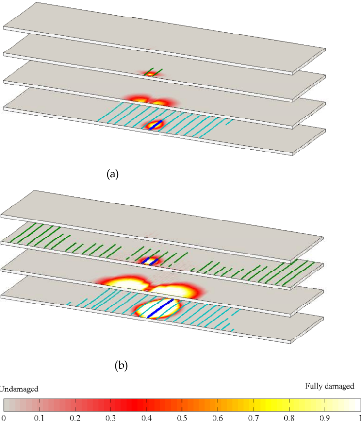
Figure 9: Damage development at two different load steps in a four-ply laminated plate; (a) Load, P = 135\text{N} , (b) Load, P = 259.2\text{N} .
