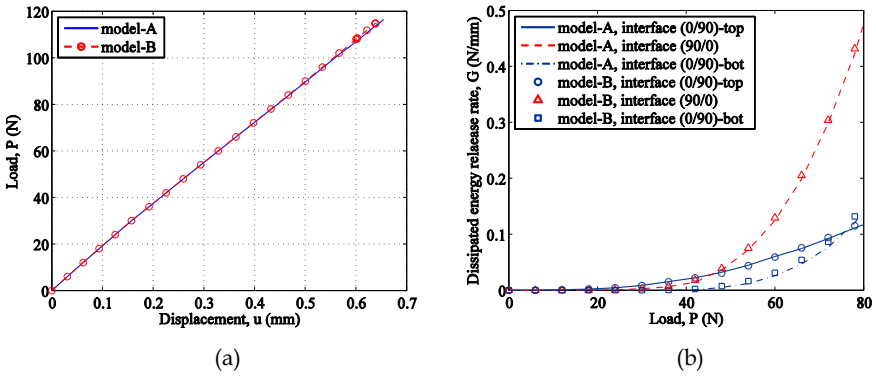
Figure 14: Four-ply laminated plate analysis results; (a) Load-displacement curves, (b) Energy dissipation due to delamination
