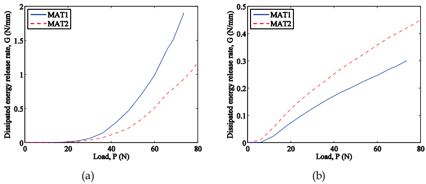
Figure 18: Energy dissipation in a two-ply laminated plate with different material properties; (a) Delamination energy dissipation, (b) Matrix cracking energy dissipation
