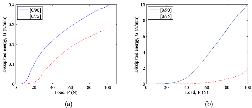
Figure 13: Energy dissipation due to matrix cracking and delamination damage in a two-ply laminate with stacking sequence [0/90] and [0/75]; (a) Energy dissipation due to matrix cracking, (b) Energy dissipation due to delamination.
