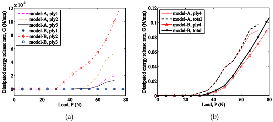
Figure 15: Energy dissipation due to matrix cracking in different plies of four-ply laminated plate
