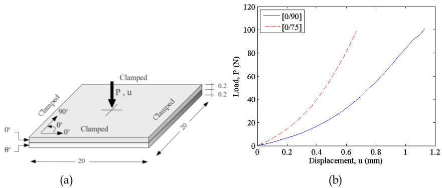
Figure 11: Two-ply model geometry and analysis results; (a) Model geometry and boundary conditions, (b) Load-displacement curves
