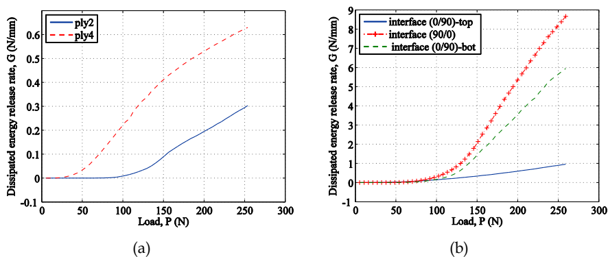
Figure 8: Energy dissipation during matrix cracking and delamination damage in a four-ply laminated plate; (a) Energy dissipation due to matrix cracking, (b) Energy dissipation due to delamination.
