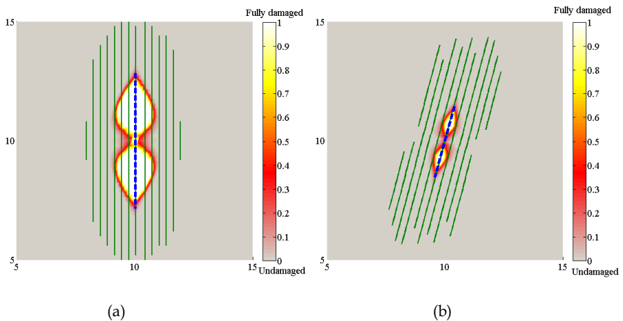
Figure 12: Matrix cracking in the lower ply and delamination damage at the interface for (0/90) and (0/75) laminates - Load, P = 101\text{N} ; (a) [0/90] laminate, (b) [0/75] laminate.
