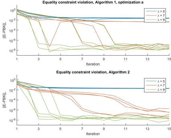
Fig. 1. The nuclear norm of the equality constraint violation, \|\mathcal{E} - \mathcal{PB}_u \mathcal{K}\|_* .
