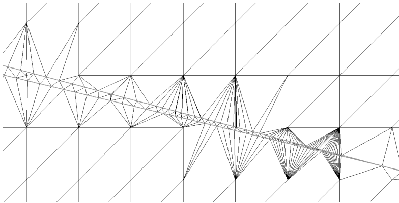
Figure 2.18: Two near-parallel lines cause addition of large numbers of Steiner points in a conforming Delaunay triangulation (Stoter et al. 2005)
