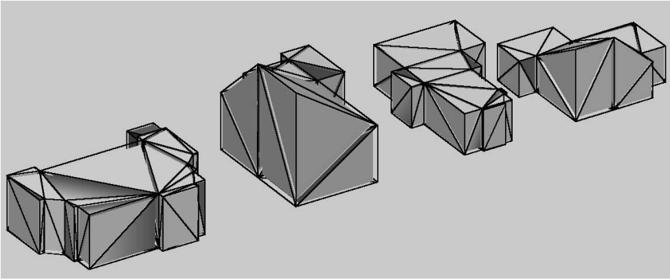
Figure 7.11: Small details such as the building extensions (less than one metre) cause less problems in case the parallel lines are not all coplanar (compared with figure 7.5)
