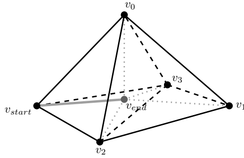
Figure 6.7: I_{02} : v_{start} is an existing node, while v_{end} lies on triangle \langle v_0, \langle v_2, v_3 \rangle . Both tetrahedrons are split into three new tetrahedrons)
