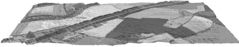
Figure 2.5: A 2.5D cadastral map: points, lines and polygons are used to model parcels and terrain elevation in 3D space
