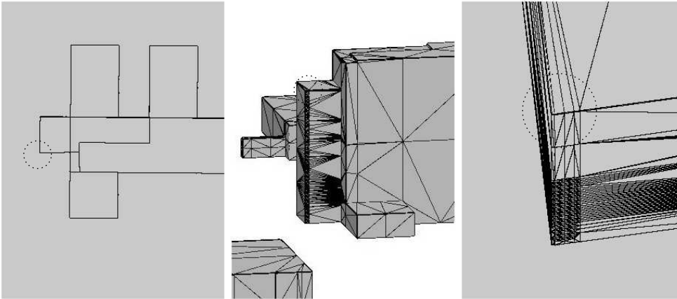
Figure 7.5: The results of improper data cleaning: unnecessary points result in close parallel lines after extrusion, thus triggering the creation of many unwanted tetrahedrons. The unnecessary points lie on the edge in the circle, but are not visible in the top view (left: top view, mid: bird’s eye view, right: detail)
