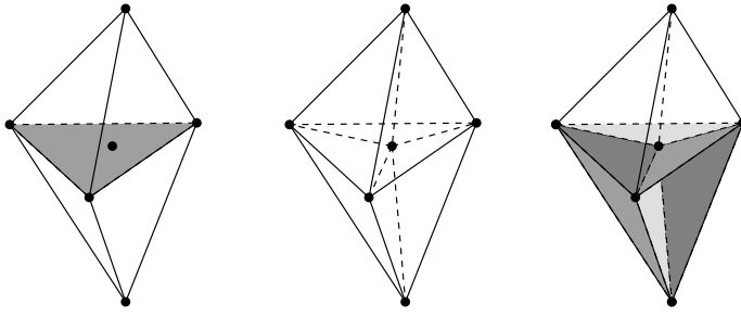
Figure 2.28: Bowson/Watson algorithm in 3D: insert a new vertex, delete tetrahedrons with non-empty circumcircles and tetrahedronise resulting hole
