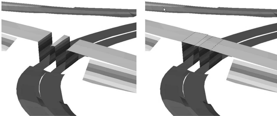
Figure 2.6: A multiple 2.5D model: two 2.5D layers are used. Left the terrain model (layer 1), right both the terrain model and the viaduct model (layer 1 + 2)
