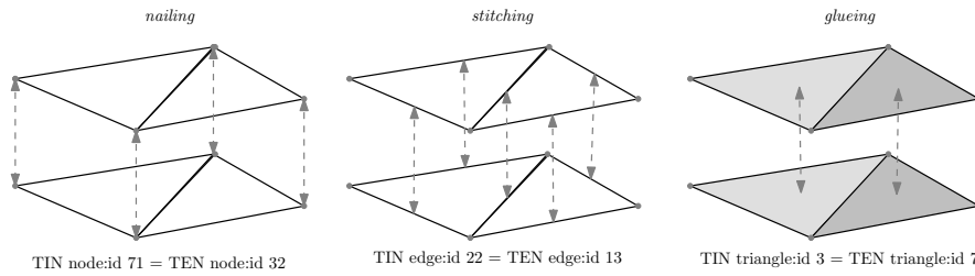
Figure 3.3: Three options for linking TIN and TENs: nailing, stitching and glueing
