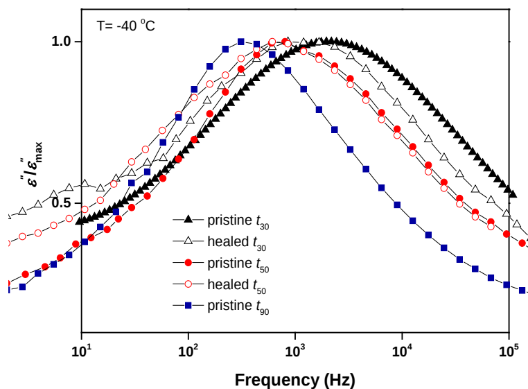
Figure 8. Normalized dielectric loss \epsilon'' vs. frequency for the segmental mode ( T = -40\text{ }^{\circ}\text{C} ) for pristine and healed NR samples vulcanized at different curing times. Filled symbols relate to pristine samples while hollow relate to healed ones.
