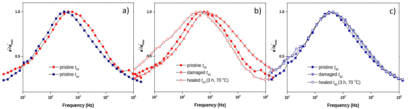
Figure 3. Normalized dielectric loss \epsilon'' vs. frequency of NR samples in the region of the segmental mode at a selected temperature ( T = -40^\circ\text{C} ) for: a) pristine 50%- and 90%-cured; b) pristine, damaged and healed 50%-cured; c) pristine, damaged and healed 90%-cured.
