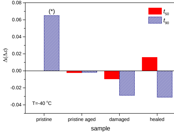
Figure 5. Dielectric strength difference \Delta(\Delta\epsilon) for 50%- and 90%-cured NR at T=-40 °C under different conditions: pristine, pristine aged, damaged, and healed. (*) Value calculated as \Delta\Delta\epsilon = \Delta\epsilon_{\text{pristine 90\%}} - \Delta\epsilon_{\text{pristine 50\%}} .
