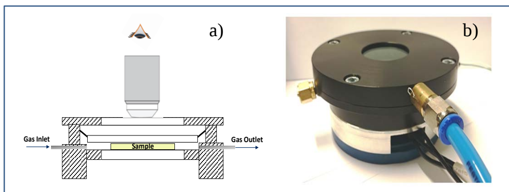
Figure 1. Home-built pressurized healing cell: a) cross-section; b) final set-up.
