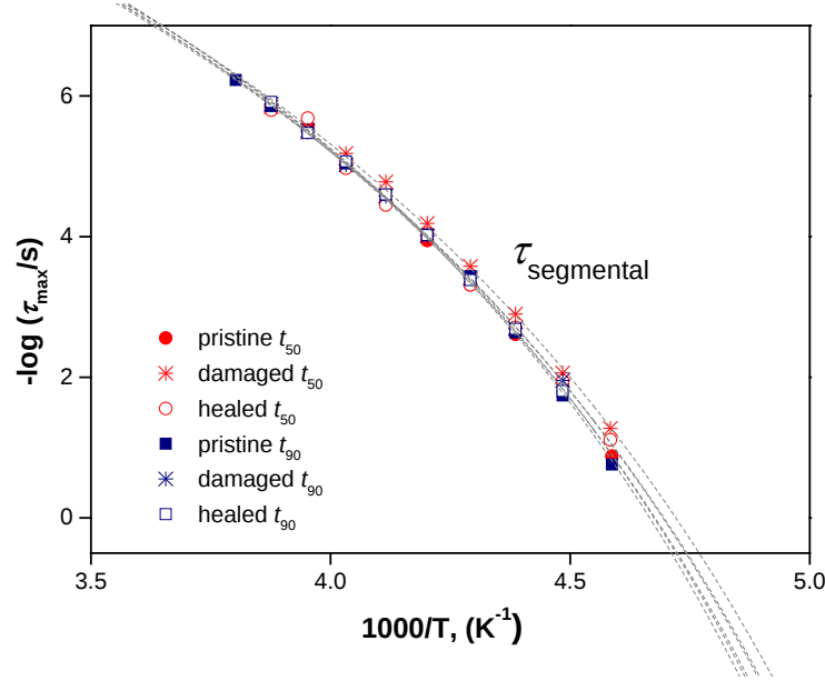
Figure 6. Temperature dependence of the average relaxation time for the segmental mode of pristine, cyclic damaged and healed NR samples vulcanized at different curing times. Dotted lines correspond to the VFT fit.
