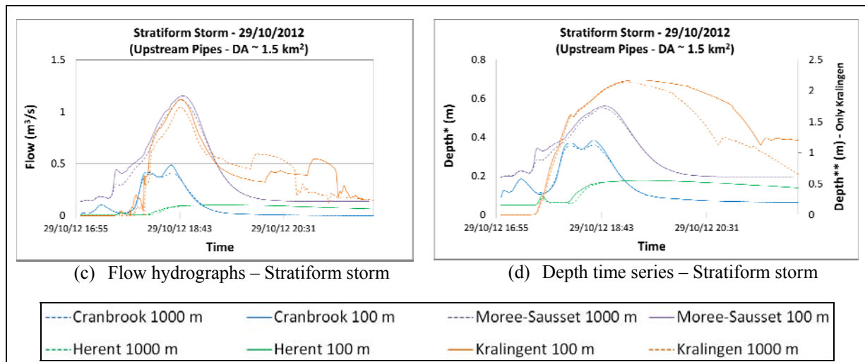
Figure 2: Response hydrographs and water depths at the downstream end of the upstream pipes selected for analysis at each pilot location (with drainage area (DA) ~ 1.5 km 2 ). The solid lines correspond to the 100 m resolution outputs and the dashed lines to the 1000 m ones. * Water depth scale used for depths observed in Cranbrook (UK), Morée-Sausset (FR) and Herent (BE) pilot locations; **Water depth scale used for Kralingen (NL) pilot location.
