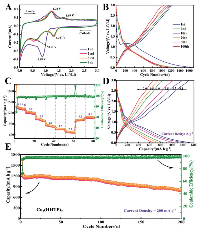
Fig. 7 Electrochemical lithium storage performance of Co-CAT MOF: (A) CV curves of Co-CAT MOF at 0.1\text{ mV s}^{-1} ( 0.01\text{--}3.0\text{ V} ). (B) Discharge-charge plots for different cycles at 200\text{ mA g}^{-1} . (C) Rate performance of Co-CAT MOF. (D) Discharge-charge profiles of Co-CAT MOF at different current densities. (E) Cycle performance at a current density of 200\text{ mA g}^{-1} .
