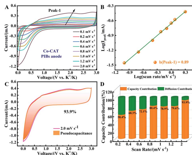
Fig. 5 Pseudocapacitive performance of the Co-CAT MOF electrode for PIBs. (A) CV profiles of the Co-CAT MOF with different scan rates. (B) Correlation between \log(i_{\text{peak}}/\text{mA}) and \log(\text{scan rate}/\text{mV s}^{-1}) . (C) Contribution of the pseudocapacitance of the Co-CAT MOF electrode at the scan rate of 2.0 \text{ mV s}^{-1} . (D) Capacity-/diffusion-contribution ratio of Co-CAT MOF with different scan rates.
