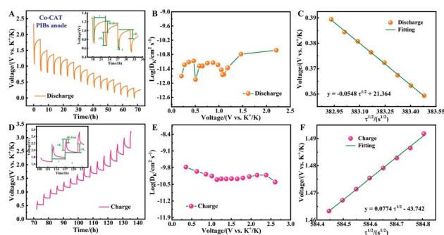
Fig. 4 GITT curves of the Co-CAT MOF electrode for the (A) discharge and (D) charge processes in the initial cycle at 100 \text{ mA g}^{-1} . The variation of D_{K^+} during (B) discharge and (E) charge processes. The corresponding linear behavior of voltage and t^{1/2} during (C) discharge and (F) charge processes.
