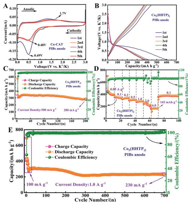
Fig. 3 Electrochemical performance of the Co-CAT MOF electrode for potassium-ion storage: (A) CV profiles of Co-CAT MOF at 0.1 mV s -1 . (B) Galvanostatic discharge/charge curves at a current density of 200 mA g -1 . Cycle stability tested at a current density of (C) 500 mA g -1 . (D) Rate performances of the Co-CAT MOF electrode. (E) Long-term stability tests at a high current density of 1000 mA g -1 .
