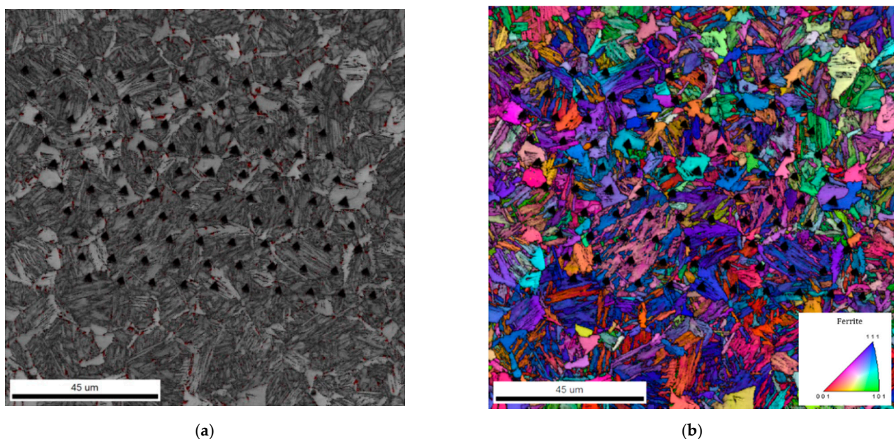
Figure 23. The Q&P sample austenitized intercritically at 800^\circ\text{C} , quenched at 318^\circ\text{C} and partitioned at 400^\circ\text{C} for 100 s. (a) 10 \times 10 mesh of the nanoindentations superimposed on a phase identification map (BCC in gray and FCC in red); (b) grid grain map for the nanoindentations mesh.
