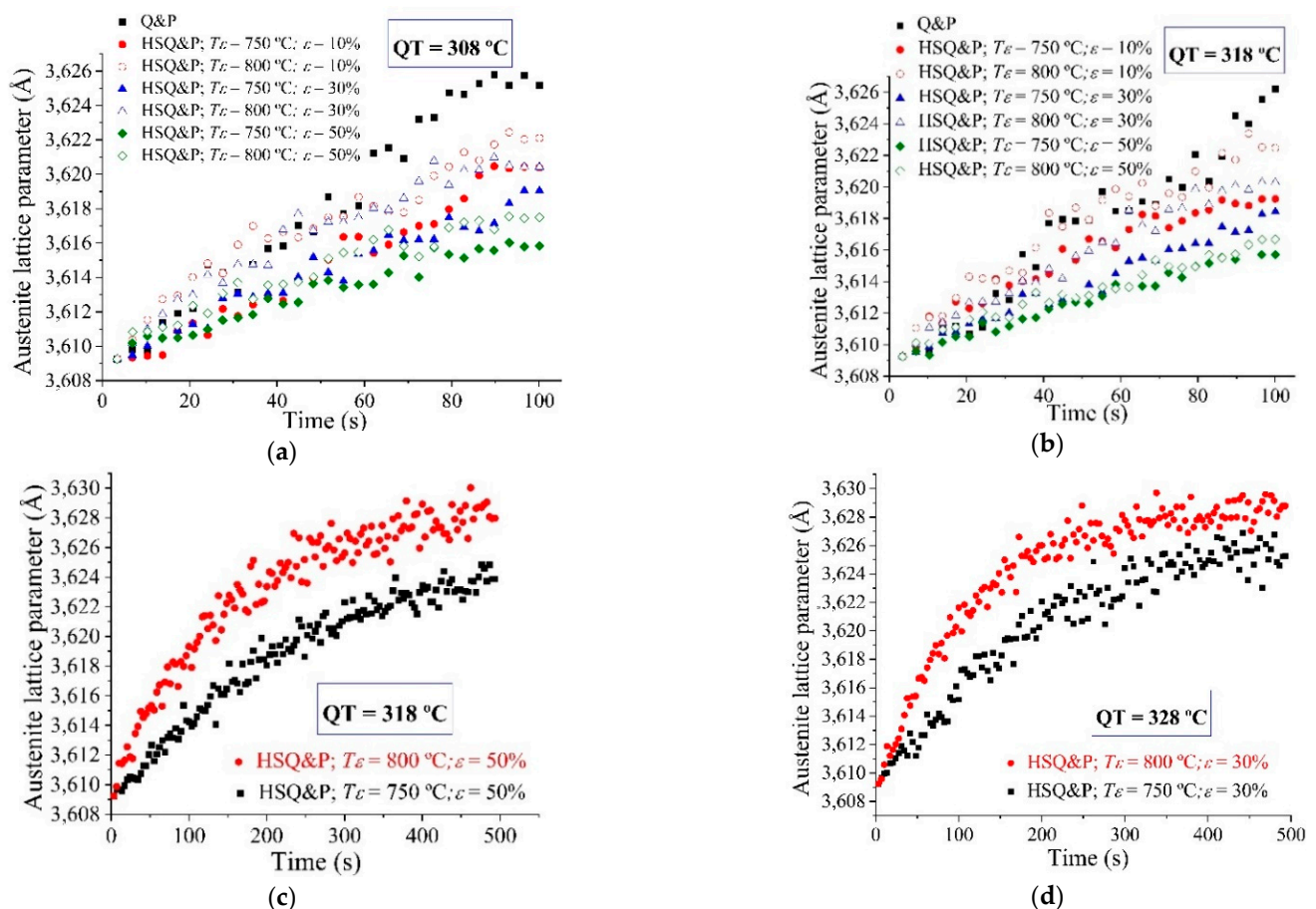
Figure 6. In situ synchrotron X-ray diffraction analysis of the evolution of the austenite lattice parameter during the partition stage. Q&P with I-HSQ&P ( T_{\varepsilon} = 800 °C) and NI-HSQ&P ( T_{\varepsilon} = 750 °C). (a) Quenching Temperature (QT) at 308 °C, (b) QT at 318 °C by 100 s, (c) QT at 318 °C by 500 s, (d) QT at 328 °C by 500 s.
