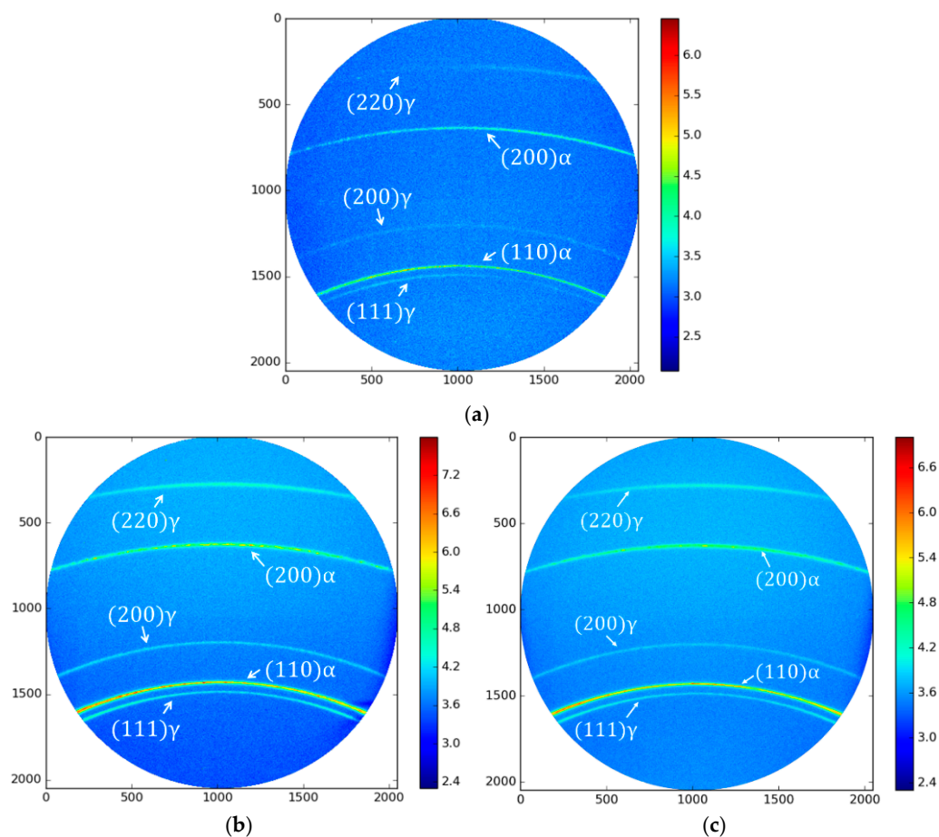
Figure 5. In situ synchrotron X-ray diffraction patterns obtained with a 2D detector showing the evolution of austenite ( \gamma ) and ferrite ( \alpha ) diffraction peaks, collected at room temperature before treatment and at 400 °C as a function of partition time (100 s). (a) as-received ( V_\gamma = 3.1\% ); (b) the initial stage of the partition ( V_\gamma = 17.2\% ); (c) final stage of the partition ( V_\gamma = 8.4\% ).
