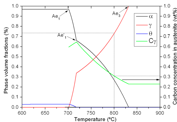
Figure 1. Phase volume fractions and carbon concentration in austenite as a function of temperature.
