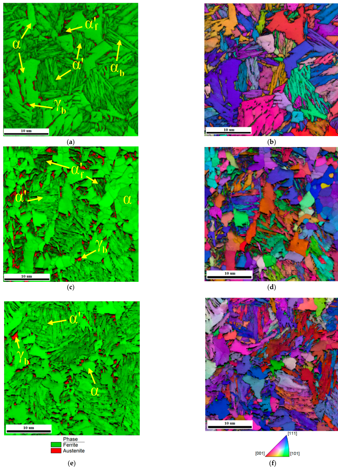
Figure 16. Images obtained by EBSD combining the tools for phase identification and grain orientation maps (IPF, images b,d,f ) of the TRIP steel samples after quenching and partition treatments (Q&P) and hot stamping followed by quenching and partition (HSQ&P) of the austenitized samples intercritically at 800 °C, quenched at 318 °C and partitioned at 400 °C for 100 s. ( a,b ) Q&P with 3.3% of γ; ( c,d ) HSQ&P with 30% deformation at 750 °C with austenite with 7.8% of γ; ( e,f ) HSQ&P with 30% deformation at 800 °C with 5.0% of γ. α', α, α b , α' f and γ represent martensite, ferrite, bainitic-ferrite, fresh martensite, and austenite, respectively.
