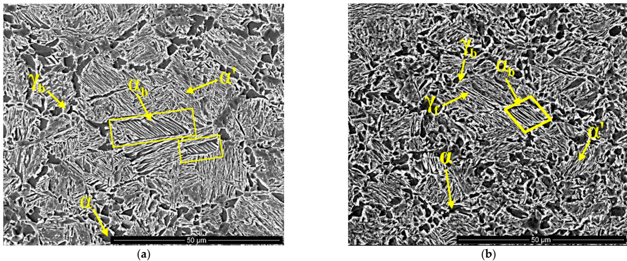
Figure 14. Microstructure (SEM) of TRIP steel samples after the combined hot stamping treatments followed by quenching and partitioning (HSQ&P) of the samples partitioned at 400 °C for 500 s. (a) HSQ&P, with 30% deformation at 800 °C and quenching temperature (QT) of 328 °C; (b) HSQ&P, with 30% deformation at 800 °C and quenching temperature (QT) of 318 °C.
