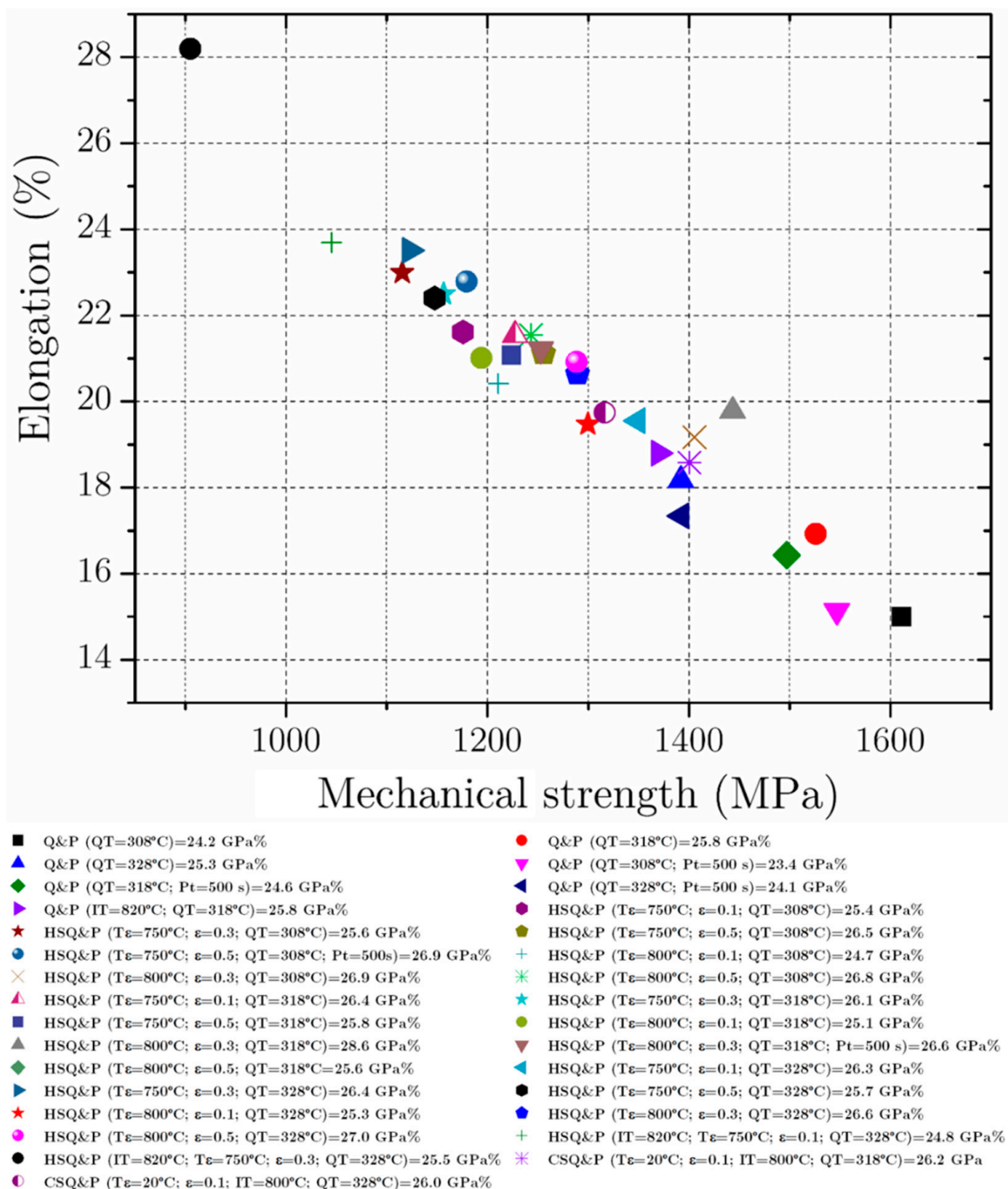
Figure 32. Combinations of ductility and mechanical strength obtained by the Mileiko model [116] using the results of the volume fractions calculated experimentally for the various heat treatments performed: quenching and partitioning (Q&P), hot stamping followed by quenching and partitioning (HSQ&P), and cold stamping followed by quenching and partition (CSQ&P). T ε , ε, QT and Pt represent the deformation temperature, the percentage of deformation, the quenching temperature, and the partitioning time, respectively.
