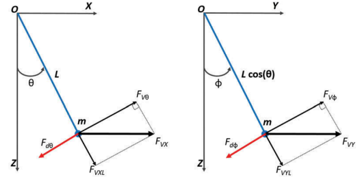
(a) Forces on the XZ plane.
