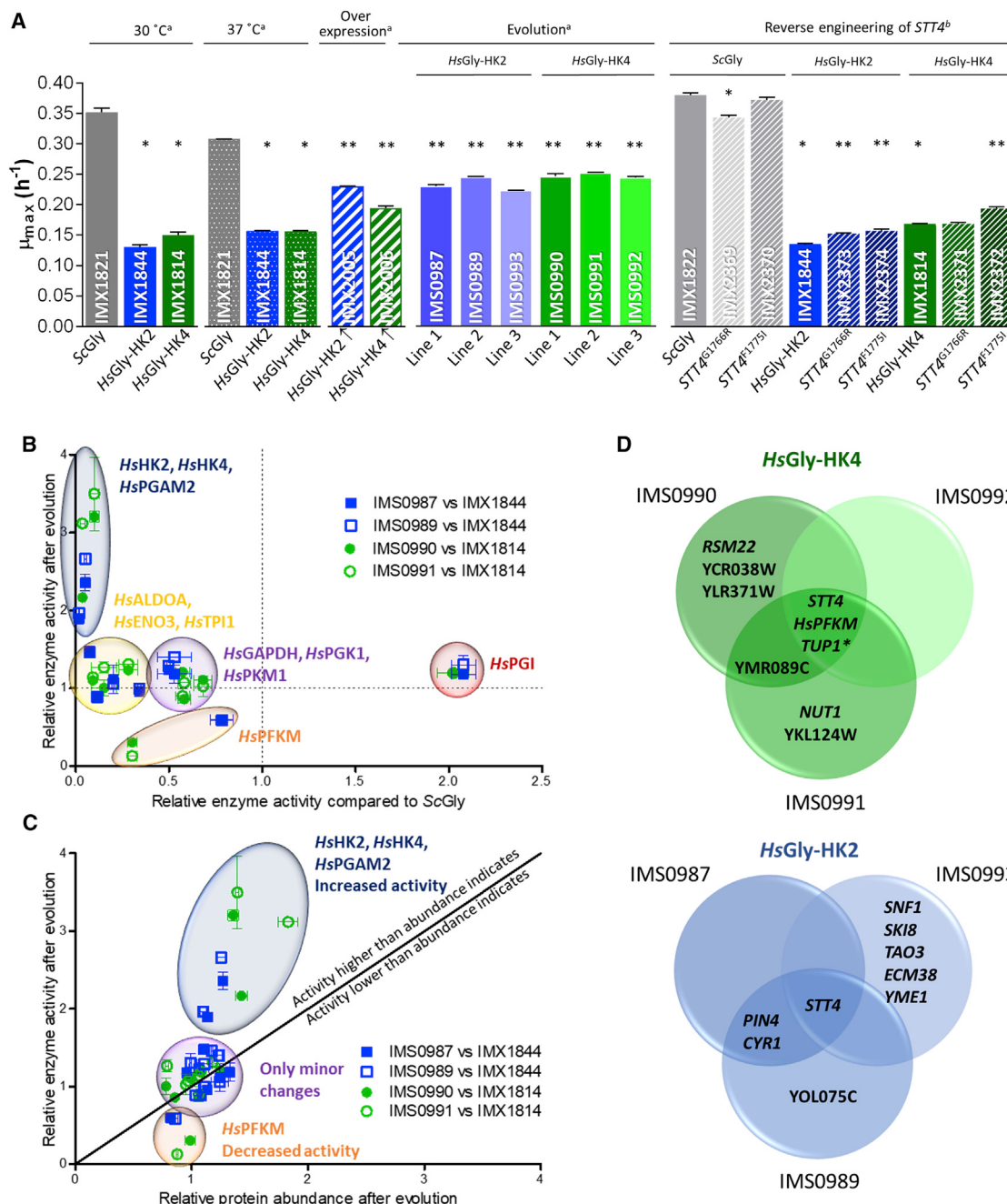
Figure 5. Strategies to improve the growth rates of fully humanized yeast strains
