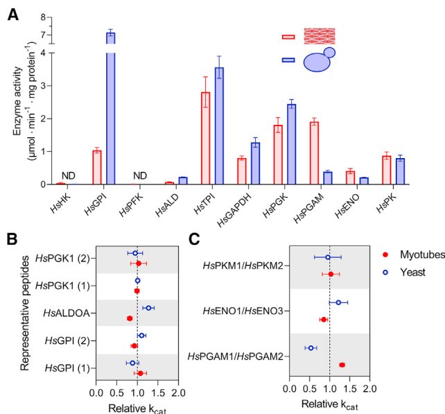
Figure 6. Enzyme activity and k_{\text{cat}} of human glycolytic enzymes in human myotubes and humanized yeast
