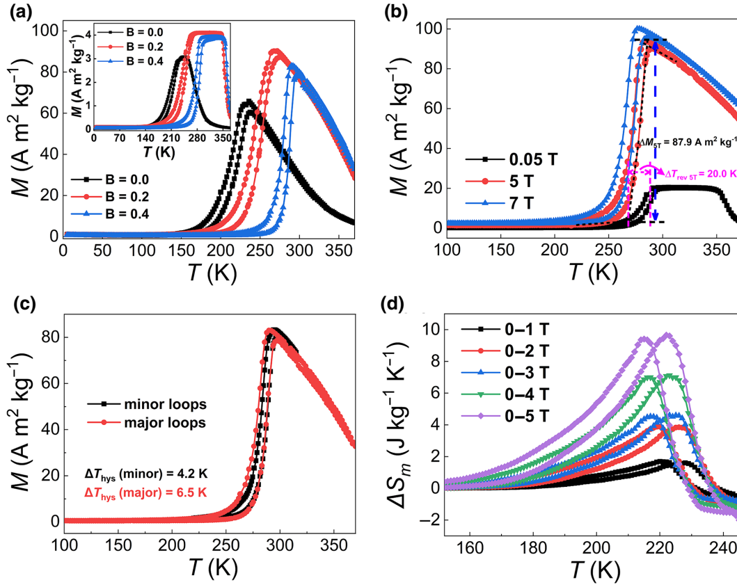
FIG. 2. (a) M - T curves measured in 1 T for \text{Ni}_{36.5}\text{Co}_{13.5}\text{Mn}_{35}\text{Ti}_{15}\text{B}_x ( x = 0.0, 0.2, 0.4 ) alloys. The inset corresponds to the M - T curves at 0.01 T. (b) M - T curves for \text{Ni}_{36.5}\text{Co}_{13.5}\text{Mn}_{35}\text{Ti}_{15}\text{B}_{0.4} in applied magnetic fields of 0.05, 5, and 7 T. The determination of \Delta M is illustrated in the figure. (c) M - T curves of \text{Ni}_{36.5}\text{Co}_{13.5}\text{Mn}_{35}\text{Ti}_{15}\text{B}_{0.4} for minor and major hysteresis loops in different temperature ranges at 1 T. (d) \Delta S_m of \text{Ni}_{36.5}\text{Co}_{13.5}\text{Mn}_{35}\text{Ti}_{15} as a function of temperature for both heating and cooling, determined in magnetic fields ( \Delta\mu_0 H ) ranging from 1 to 5 T.
