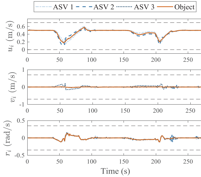
(b) Linear and angular velocities of the ASVs and the object with a time-varying configuration.
