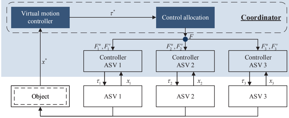
Figure 5.3: Multi-layer DMPC for cooperative object transport.
