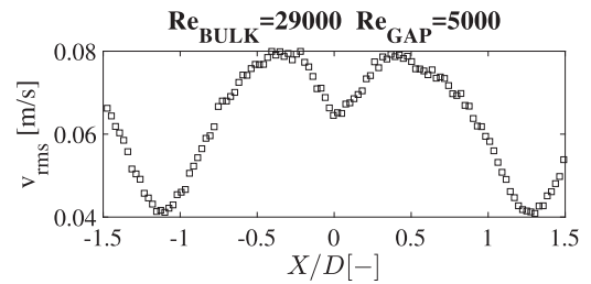
Fig. 10. v_{rms} profile along the gap; P/D = 1.2 . The profile looks symmetric even with the highest flow rate: the larger gap, here, allows the lateral momentum component of the flow to redistribute between the two sub-channels.
