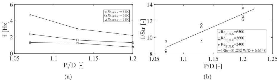
Fig. 22. (a): Average span-wise frequency against P/D for three Re numbers. (b): 1/Str against P/D : experimental results and proposed correlation.
