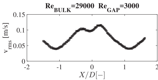
Fig. 8. v_{rms} profile along the gap; P/D = 1.07 . The asymmetry is due to the lateral momentum component of the flow in the main sub-channels.
