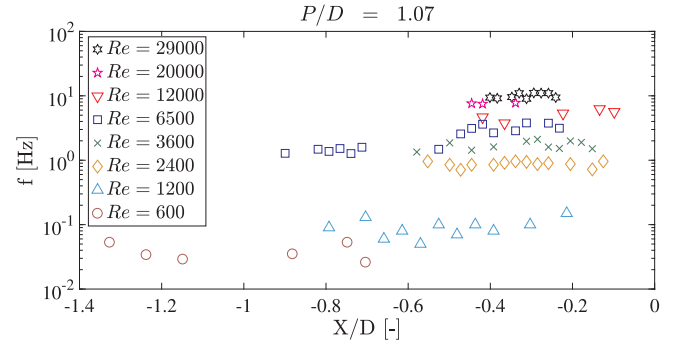
Fig. 23. Average stream-wise frequency of the flow structures and their locations for the investigated Re ; P/D = 1.07 . As Re_{BULK} increases the structures move further inward into the gap and they appear less scattered.
