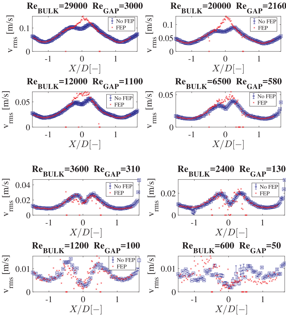
Fig. 31. Measurement of v_{rms} along path A FEP (red series) and along path A no-FEP from the second side (blue series); P/D = 1.07 . The effect of a too small gap, compared to the probe size, is the central peak due to reflection of light and contact between the measurement volume and the walls; it is interpreted by the software as zero-velocity signal. (For interpretation of the references to colour in this figure legend, the reader is referred to the web version of this article.)
