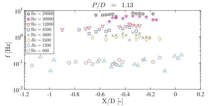
Fig. 24. Average stream-wise frequency of the flow structures and their locations for the investigated Re ; P/D = 1.13 .
