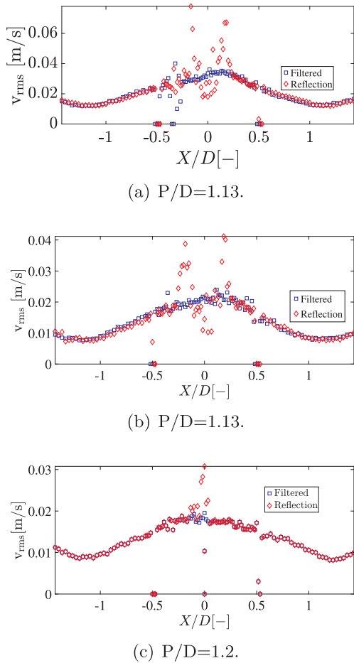
Fig. 34. Comparison between the v_{rms} affected by light reflection from the wall (red) and filtered (blue). The reflection can be corrected with a filter on the measured velocity provided this is sufficiently higher than zero. (a): Re_{BULK} = 6500 , Re_{GAP} = 880 ; (b): Re_{BULK} = 3600 , Re_{GAP} = 400 ; (c): Re_{BULK} = 3600 , Re_{GAP} = 600 . (For interpretation of the references to colour in this figure legend, the reader is referred to the web version of this article.)
