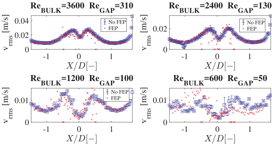
Fig. 32. v_{rms} along the gap through the FEP (red series) and from the second side (blue series); P/D = 1.07 . (For interpretation of the references to colour in this figure legend, the reader is referred to the web version of this article.)
