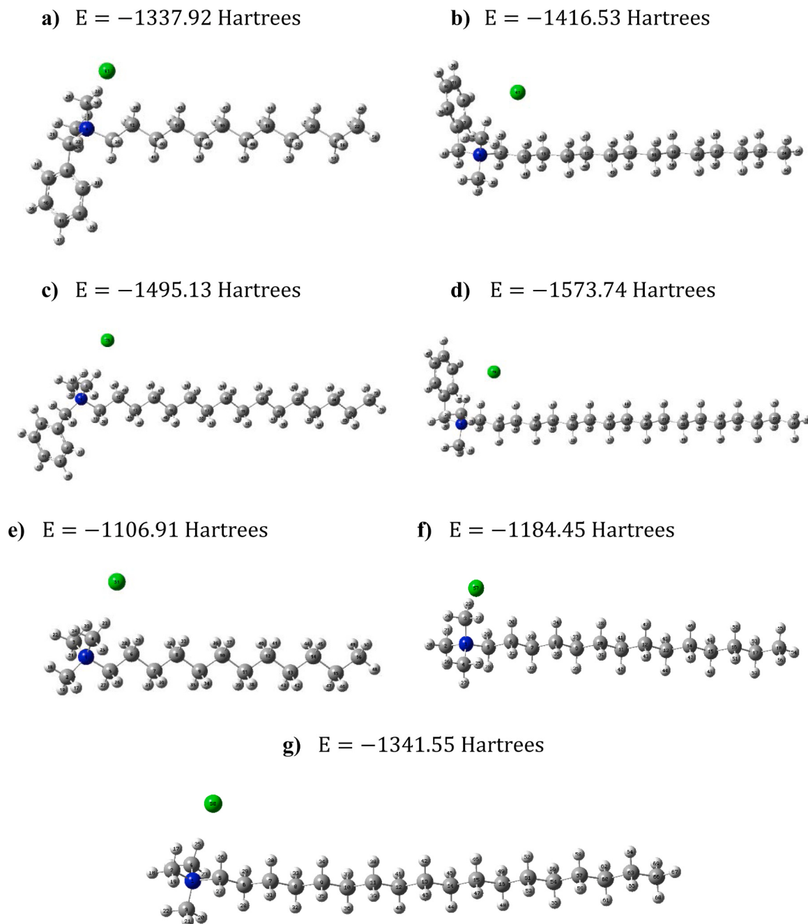
Fig. 1. Structure and electronic energy ( E ) without zero point energy correction for selected QACs at M06–2X/6–311 G(d,p) level of theory: a) BAC C12, b) BAC C14, c) BAC C16, d) BAC C18, e) ATMAC C12, f) ATMAC C14 and g) ATMAC C18. Hydrogen, carbon, nitrogen, and chlorine atoms are represented by white, gray, blue, and green spheres, respectively.
