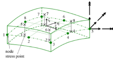
Figure 8.3: The quadrilateral shell element SCQS with stress points [31]
