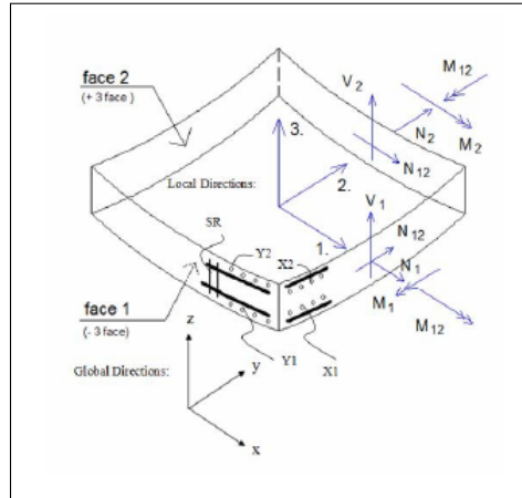
Figure 9.2: Reinforcement directions [32]
