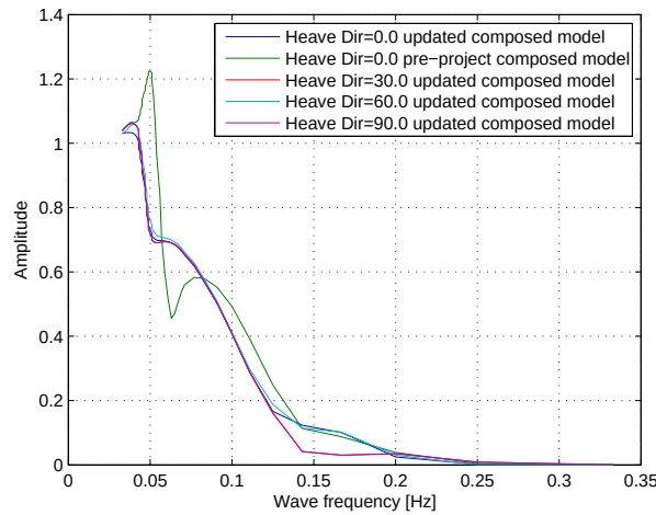
Figure 7.4: Heave RAO
