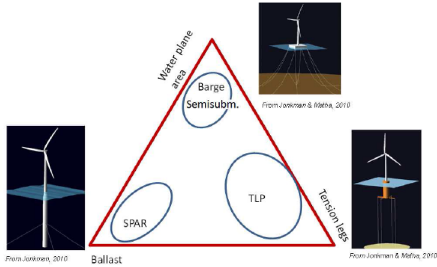
Figure 1.2: Classification of floaters [10]
