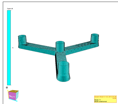
(b) 7048 Elements (7083 Nodes) panel model for the hydrodynamic analysis
