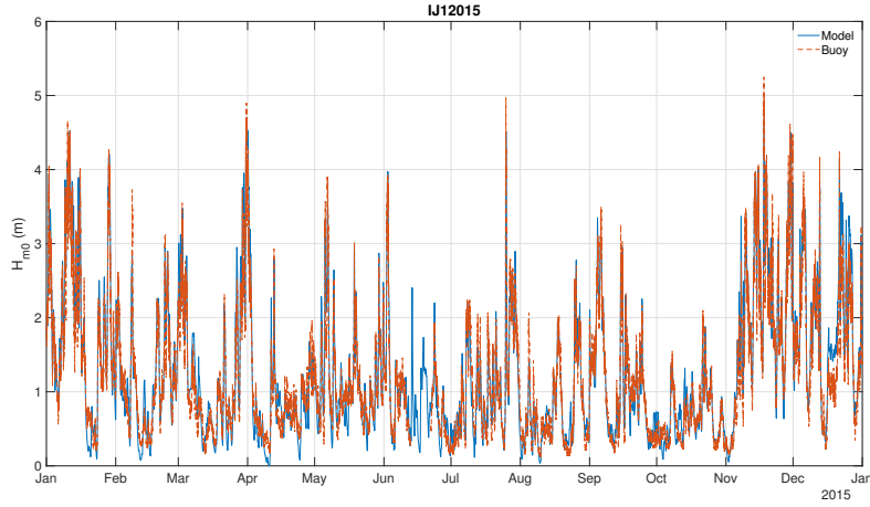
(a) In-situ vs hindcast timeseries
