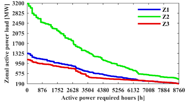
Fig. 4. Zonal active power load duration curve.
