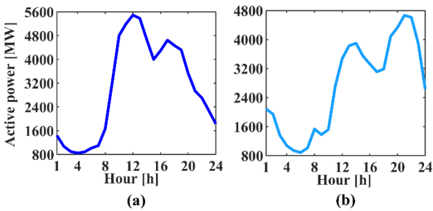
Fig. 3. The system's total power demand considers a peak load day (a) and baseload day (b).
