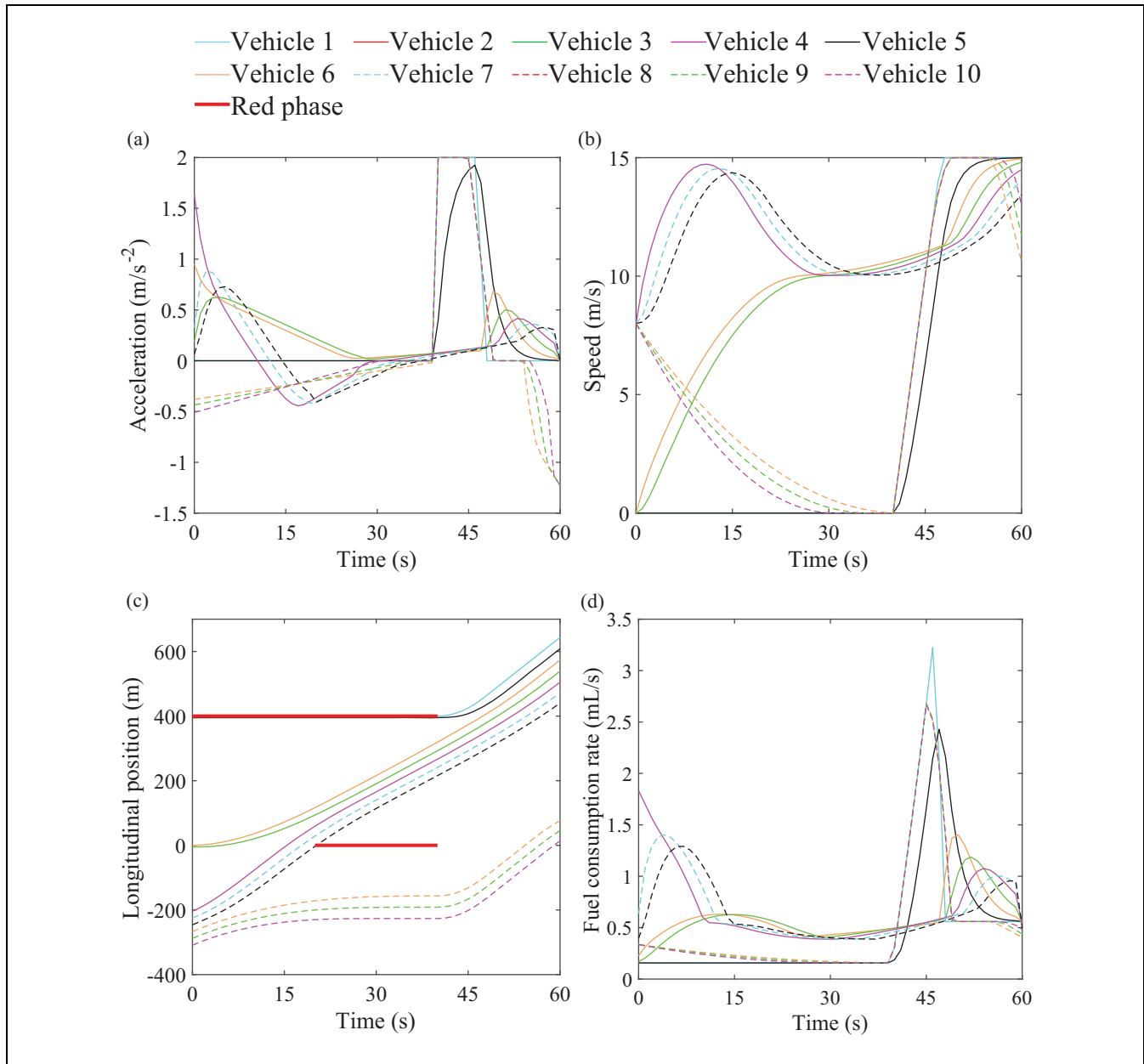
Figure 4. Optimal trajectories in Scenario 3: (a) acceleration; (b) speed; (c) longitudinal position; and (d) fuel consumption rate.
