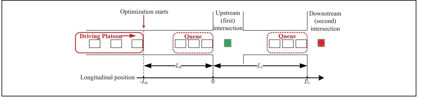
Figure 1. Illustration of operation of the control system.
