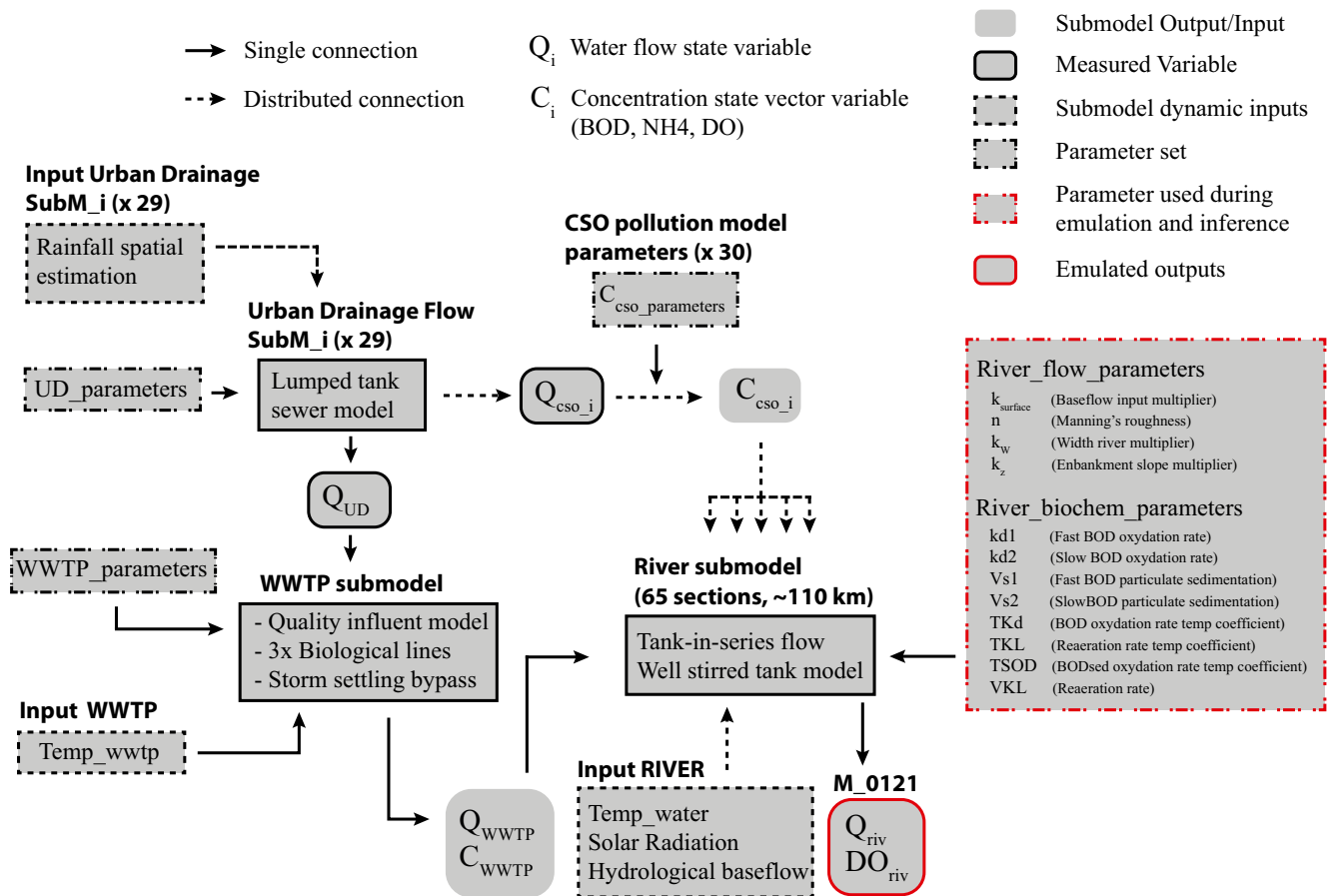
Fig. 14 Model scheme
