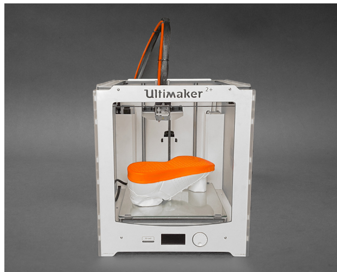
Figure 7. Shoe exploration #3 Replenishing AB plastic sole (in orange) with a 3D printer.
