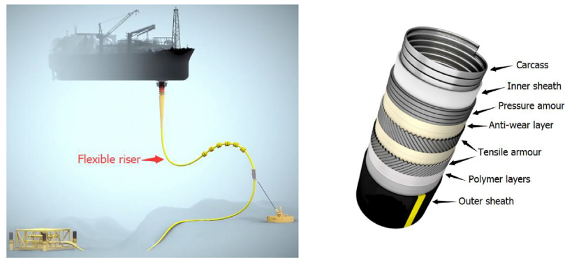
Fig. 1. Flexible riser and its layer configuration.
